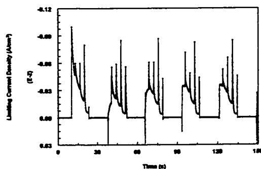
Figure 4.1.3 Instantaneous limiting current density for 0.03 Hz bubble in electrochemical cell
