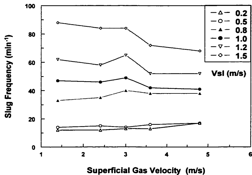
Figure 4.3.1.1 Effect of superficial gas velocity on the slug frequency
