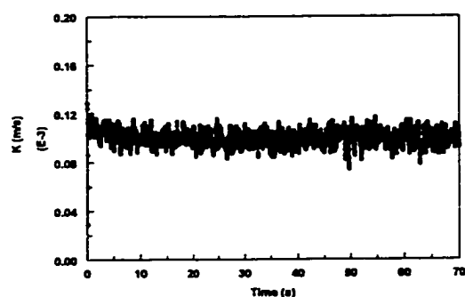
Figure 4.3.2.7-b Instantaneous mass transfer coefficient at V_{sl}=1.0 m/s and V_{sg}=0.4 m/s in water/gas/oil flow with 20% oil
