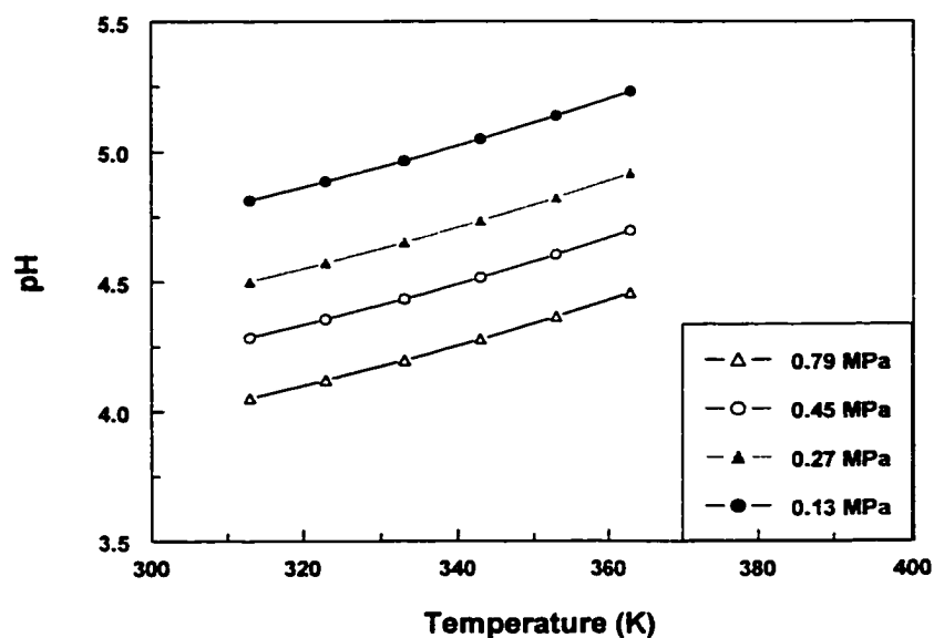
Figure 6.1.1 Predicted pH vs temperature and pressure for brine
