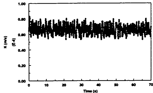
Figure 4.3.1.8-d Instantaneous mass transfer coefficient at V_{sl}=1.0 m/s and V_{sg}=0.8 m/s in water/gas flow
