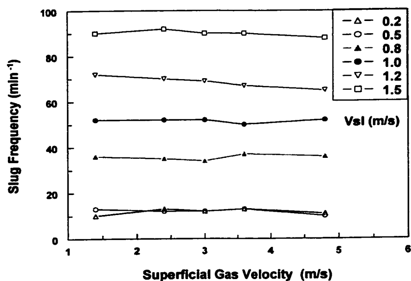
Figure 4.3.2.1 Effect of superficial gas velocity on the slug frequency with 20% input oil
