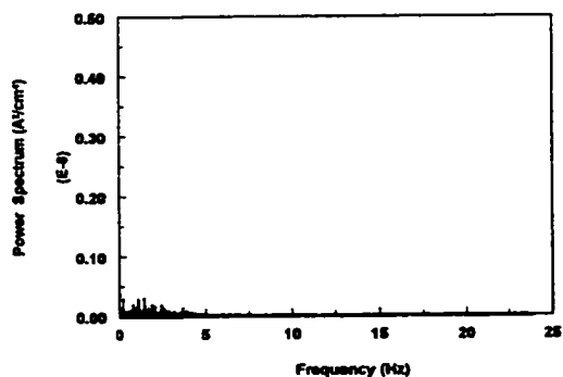
Figure 4.1.16 Power spectrum of the instantaneous limiting current density in full pipe flow with V_{sl}=1.5 m/s
