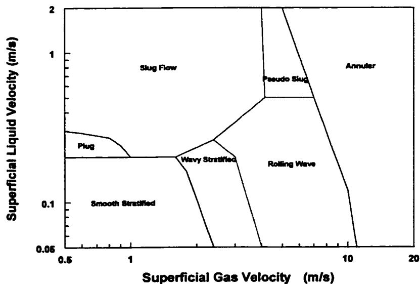
Figure 2.5 A typical flow regime map for gas/oil/liquid three-phase flow in horizontal pipes (Lee, 1993)
