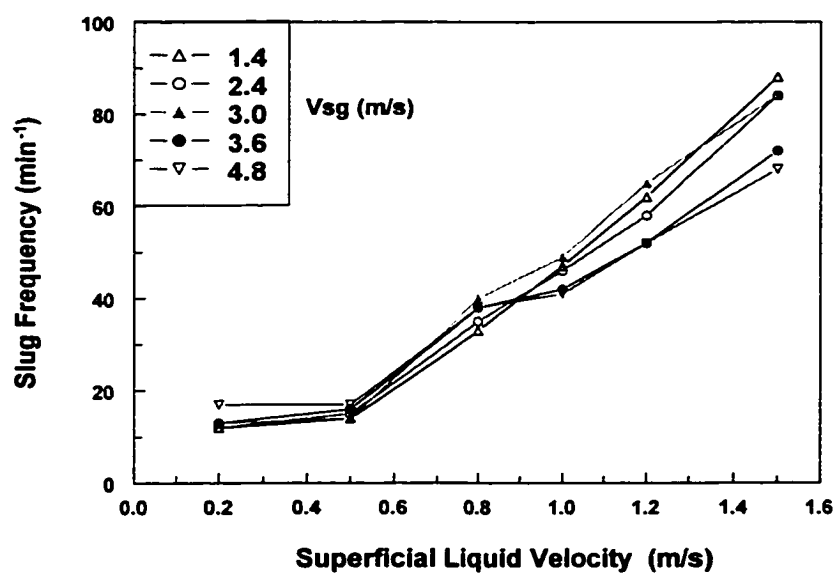
Figure 4.3.1.2 Effect of superficial liquid velocity on the slug frequency
