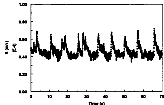
Figure 4.3.1.5-d Instantaneous mass transfer coefficient at V_{sl}=0.2 m/s and V_{sg}=0.8 m/s in water/gas flow
