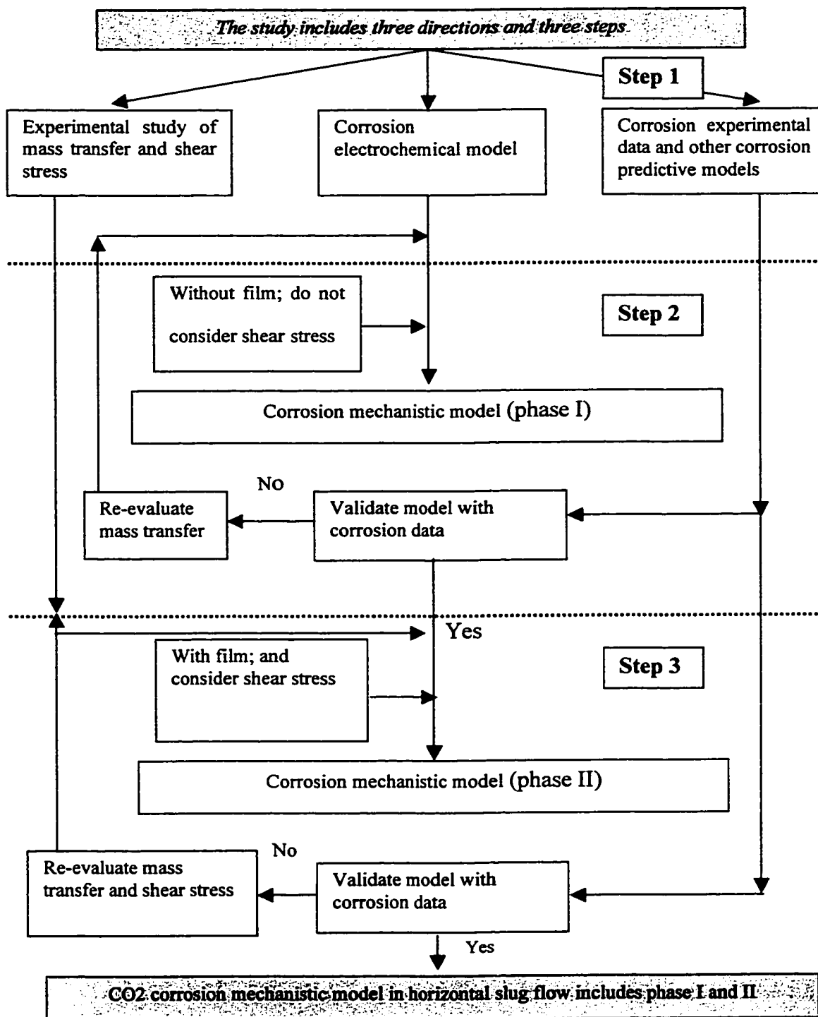
Figure 5.5.1 Development of corrosion mechanistic model for slug flow
