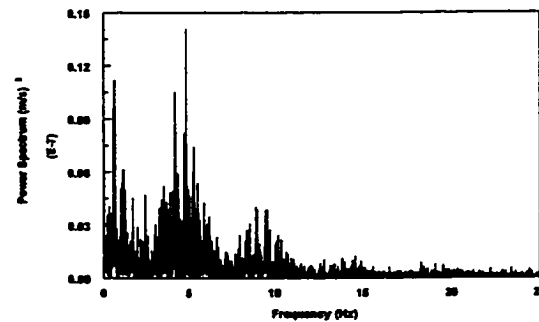
Figure 4.3.15-j Power spectrum of the instantaneous mass transfer coefficient at V_{sl}=1.2 m/s and V_{sg}=4.8 m/s in water/gas flow
