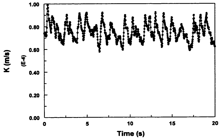
Figure 4.4.5 Instantaneous mass transfer coefficient in water/gas two-phase flow with V_{sl}=1.0 m/s and V_{sg}=1.4 m/s
