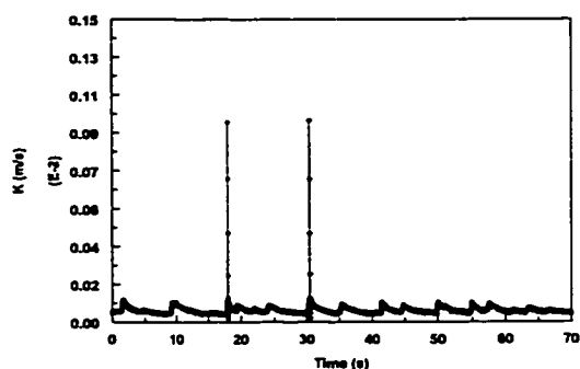
Figure 4.3.1.5-g Instantaneous mass transfer coefficient at V_{sl}=0.2 m/s and V_{sg}=2.4 m/s in water/gas flow
