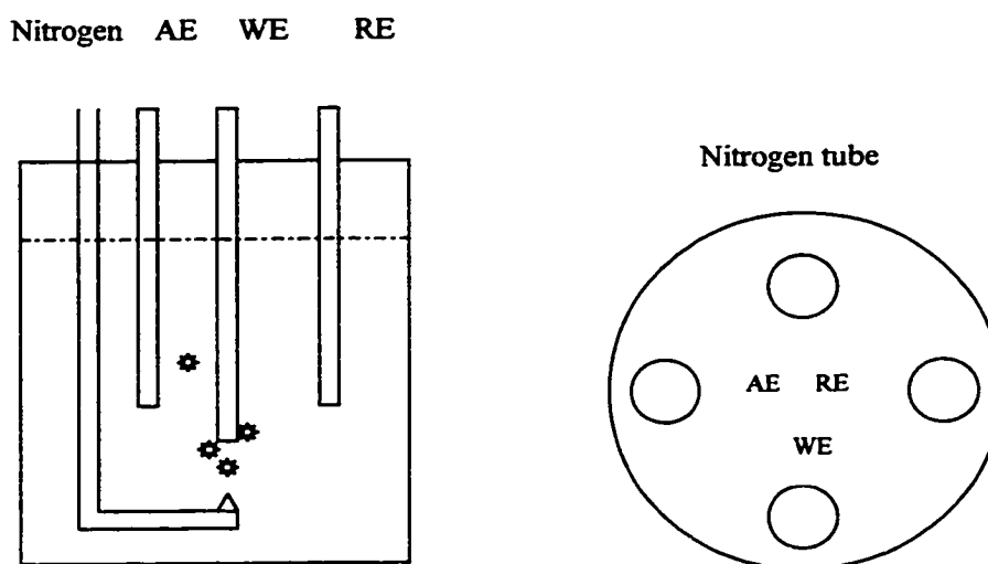
Figure 3.3 Schematic of electrochemical cell
