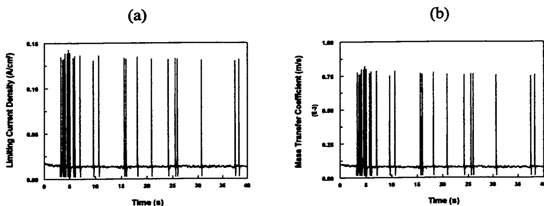
Figure 4.2.10 Instantaneous limiting current density (a) and instantaneous mass transfer coefficient (b) in water/oil flow at velocity 1 m/s
