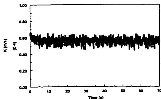
Figure 4.3.1.8-b Instantaneous mass transfer coefficient at V_{sl}=1.0 m/s and V_{sg}=0.4 m/s in water/gas flow
