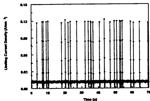
Figure 4.1.14 Instantaneous mass transfer coefficient in slug flow with V_{sl}=1.5 m/s and V_{sg}=1.4 m/s
