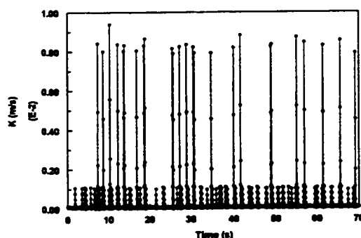
Figure 4.3.1.9-j Instantaneous mass transfer coefficient at V_{sl}=1.2 m/s and V_{sg}=4.8 m/s in water/gas flow
