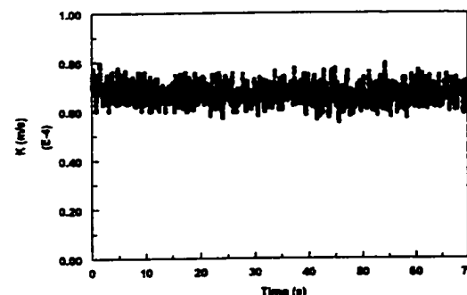
Figure 4.3.1.9-b Instantaneous mass transfer coefficient at V_{sl}=1.2 m/s and V_{sg}=0.4 m/s in water/gas flow
