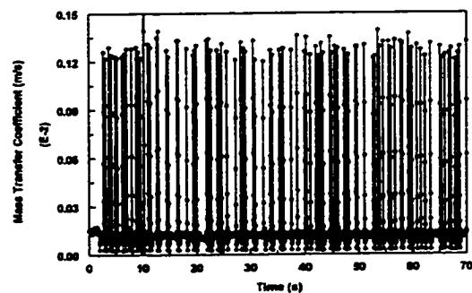
Figure 4.3.3.7-d Instantaneous mass transfer coefficient at V_{sl}=1.0 m/s and V_{sg}=0.8 m/s in water/gas/oil three-phase flow with 40% oil
