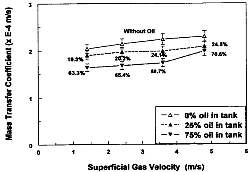
Figure 4.2.6 Average mass transfer coefficient vs superficial gas velocity in slug flow with different in situ oil percentage
