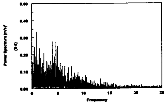
Figure 4.3.13-j Power spectrum of the instantaneous mass transfer coefficient at V_{sl}=0.8 m/s and V_{sg}=4.8 m/s in water/gas flow
