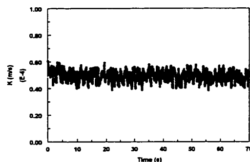
Figure 4.3.1.7-b Instantaneous mass transfer coefficient at V_{sl}=0.8 m/s and V_{sg}=0.4 m/s in water/gas flow
