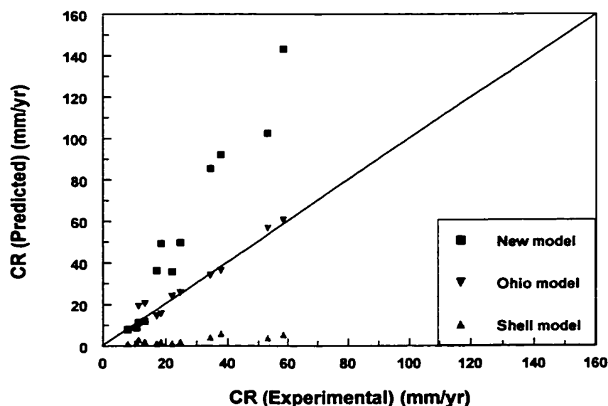
Figure 6.5.1 Comparison of three corrosion models with experimental data
