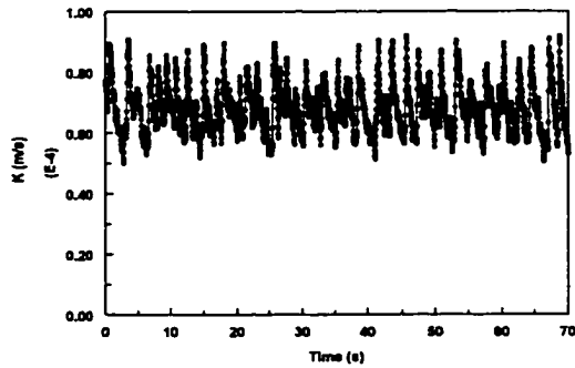
Figure 4.3.1.7-f Instantaneous mass transfer coefficient at V_{sl}=0.8 m/s and V_{sg}=1.4 m/s in water/gas flow
