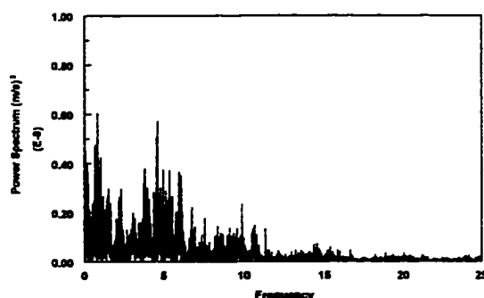
Figure 4.3.1.14-j Power spectrum of the instantaneous mass transfer coefficient at V_{sl}=1.0 m/s and V_{sg}=4.8 m/s in water/gas flow
