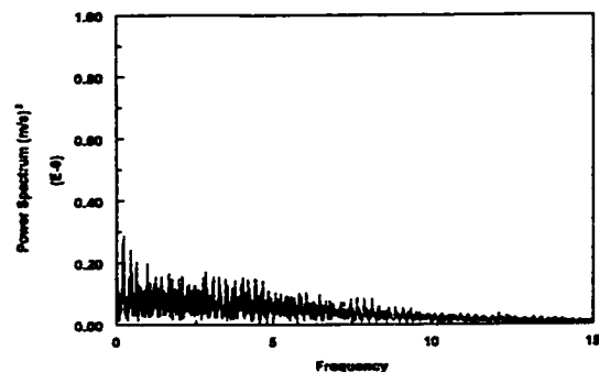
Figure 4.3.12-i Power spectrum of the instantaneous mass transfer coefficient at V_{sl}=0.5 m/s and V_{sg}=3.6 m/s in water/gas flow
