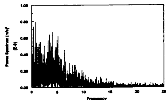
Figure 4.3.1.14-h Power spectrum of the instantaneous mass transfer coefficient at V_{sl}=1.0 m/s and V_{sg}=3.0 m/s in water/gas flow
