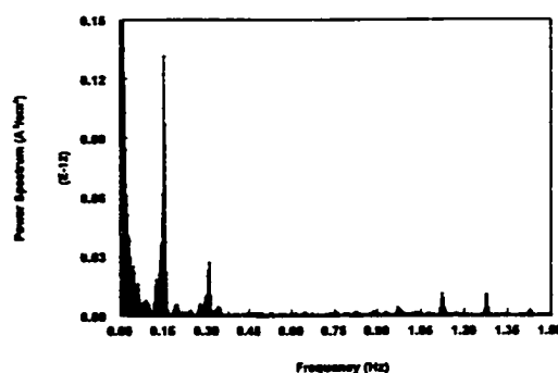
Figure 4.1.2 Power spectrum of the instantaneous limiting current density at 0.2 Hz bubble in the electrochemical cell
