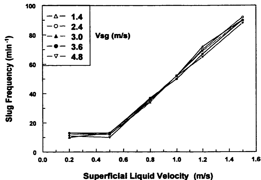
Figure 4.3.2.2 Effect of superficial liquid velocity on the slug frequency with 20% input oil
