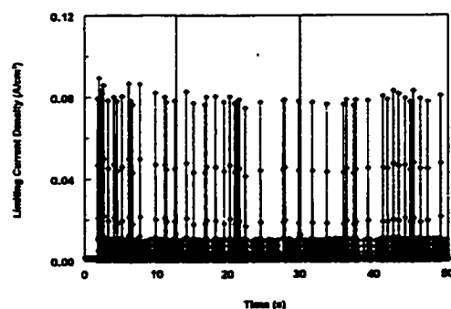
Figure 4.1.7 Instantaneous limiting current density in stationary slug with Froude 6
