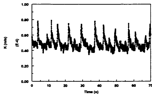
Figure 4.3.1.5-e Instantaneous mass transfer coefficient at V_{sl}=0.2 m/s and V_{sg}=1.0 m/s in water/gas flow
