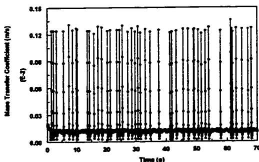
Figure 4.3.3.7-c Instantaneous mass transfer coefficient at V_{sl}=1.0 m/s and V_{sg}=0.6 m/s in water/gas/oil three-phase flow with 40% oil
