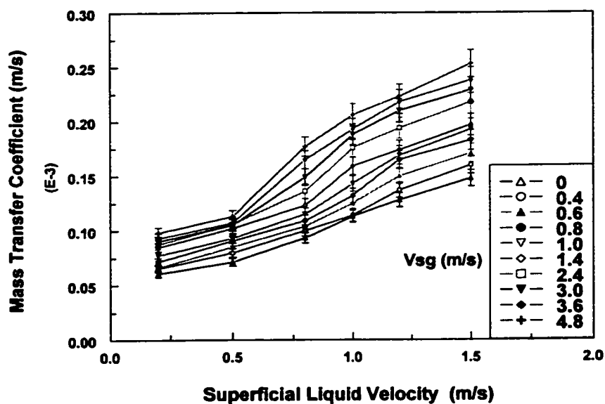
Figure 4.3.3.4 Effect of superficial gas velocity on the average mass transfer coefficient in slug flow and other flows with 40% input oil
