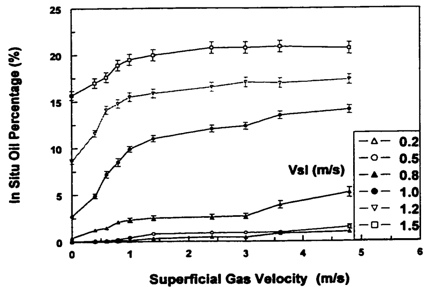
Figure 4.3.2.5 Effect of superficial gas velocity on the in situ oil percentage at the bottom of pipe in water/gas/oil three-phase flow with 20% input oil
