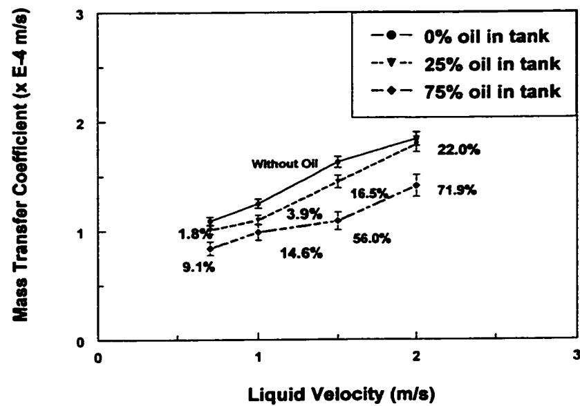
Figure 4.2.4 Average mass transfer coefficient of five electrodes vs liquid velocity in full pipe flow with different in situ oil percentage
