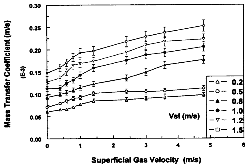
Figure 4.3.3.3 Effect of superficial gas velocity on the average mass transfer coefficient in slug flow and other flows with 40% input oil
