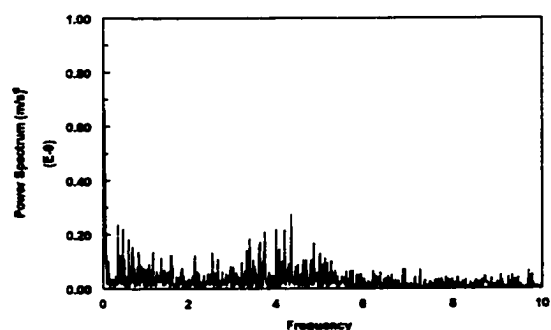
Figure 4.3.1.14-g Power spectrum of the instantaneous mass transfer coefficient at V_{sl}=1.0 m/s and V_{sg}=2.4 m/s in water/gas flow
