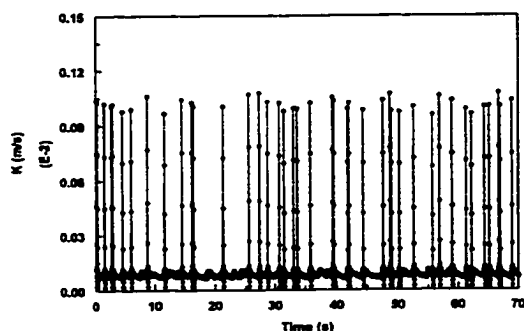
Figure 4.3.1.8-g Instantaneous mass transfer coefficient at V_{sl}=1.0 m/s and V_{sg}=2.4 m/s in water/gas flow
