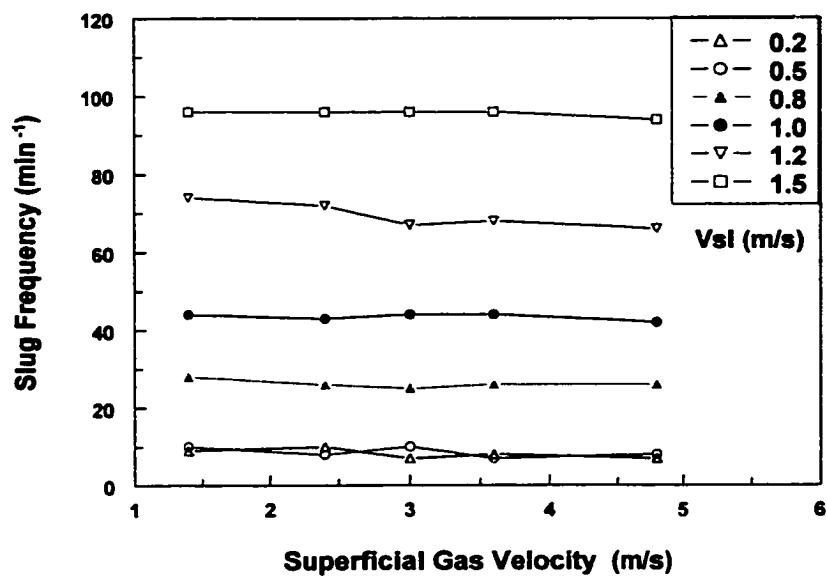
Figure 4.3.3.1 Effect of superficial gas velocity on the slug frequency with 40% input oil
