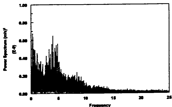
Figure 4.3.13-h Power spectrum of the instantaneous mass transfer coefficient at V_{sl}=0.8 m/s and V_{sg}=3.0 m/s in water/gas flow
