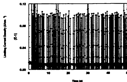
Figure 4.1.6 Instantaneous limiting current density in stationary slug with Froude 5
