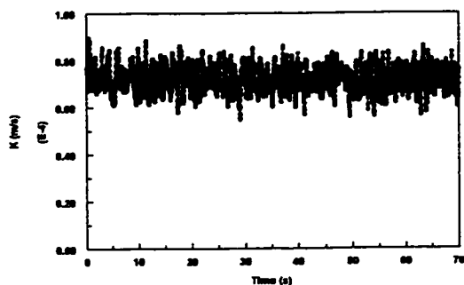
Figure 4.3.1.9-c Instantaneous mass transfer coefficient at V_{sl}=1.2 m/s and V_{sg}=0.6 m/s in water/gas flow
