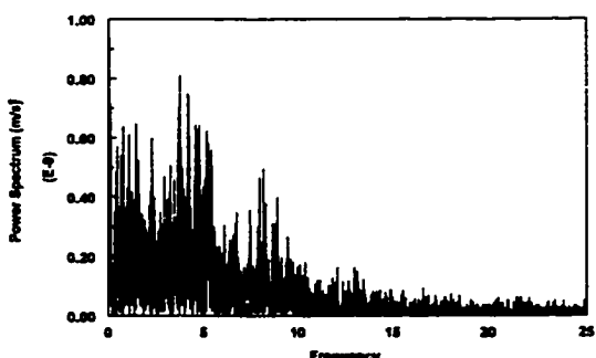
Figure 4.3.15-h Power spectrum of the instantaneous mass transfer coefficient at V_{sl}=1.2 m/s and V_{sg}=3.0 m/s in water/gas flow
