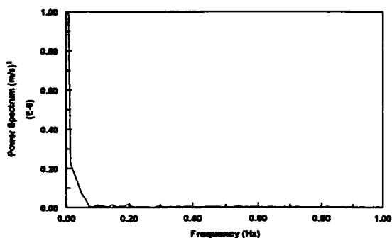
Figure 4.3.11-f Power spectrum of the instantaneous mass transfer coefficient at V_{sl}=0.2 m/s, V_{sg}=1.4 m/s in water/gas flow
