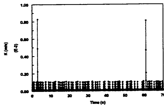
Figure 4.3.1.9-h Instantaneous mass transfer coefficient at V_{sl}=1.2 m/s and V_{sg}=3.0 m/s in water/gas flow
