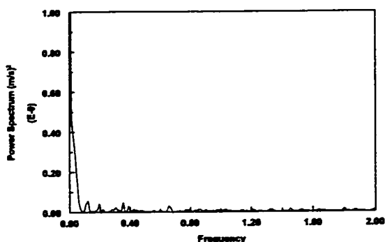
Figure 4.3.13-g Power spectrum of the instantaneous mass transfer coefficient at V_{sl}=0.8 m/s and V_{sg}=2.4 m/s in water/gas flow
