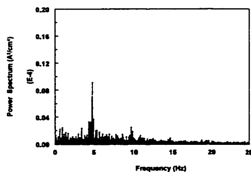
Figure 4.1.12 Power spectrum of the instantaneous limiting current density in stationary slug with Froude 7
