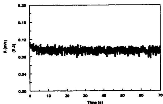
Figure 4.3.2.7-a Instantaneous mass transfer coefficient at V_{sl}=1.0 m/s and V_{sg}=0 m/s in water/gas/oil flow with 20% oil
