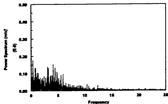
Figure 4.3.13-i Power spectrum of the instantaneous mass transfer coefficient at V_{sl}=0.8 m/s and V_{sg}=3.6 m/s in water/gas flow
