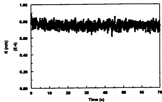
Figure 4.3.1.10-b Instantaneous mass transfer coefficient at V_{sl}=1.5 m/s and V_{sg}=0.4 m/s in water/gas flow
