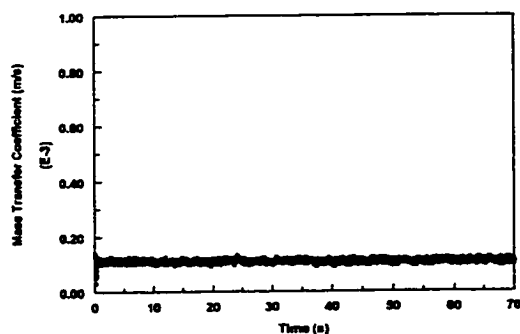
Figure 4.3.3.7-a Instantaneous mass transfer coefficient at V_{sl}=1.0 m/s and V_{sg}=0 m/s in water/gas/oil three-phase flow with 40% oil
