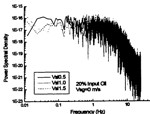
Figure 4.3.3.10 Comparison of p.s.d. at different superficial liquid velocities and 0 m/s superficial gas velocity with 20% input oil
