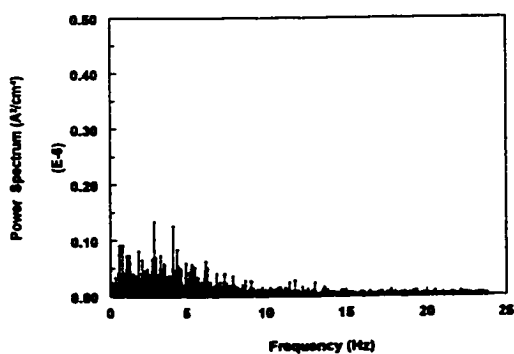
Figure 4.1.17 Power spectrum of the instantaneous limiting current density at slug flow with V_{sl}=1.5 m/s and V_{sg}=1.4 m/s
