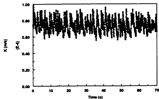
Figure 4.3.1.8-f Instantaneous mass transfer coefficient at V_{sl}=1.0 m/s and V_{sg}=1.4 m/s in water/gas flow
