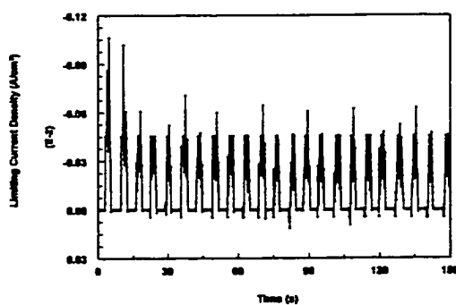
Figure 4.1.1 Instantaneous limiting current density for 0.2 Hz bubble in electrochemical cell
