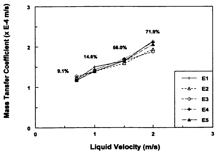
Figure 4.2.3 Local mass transfer coefficient of five electrodes vs liquid velocity in full pipe flow with 75% oil
