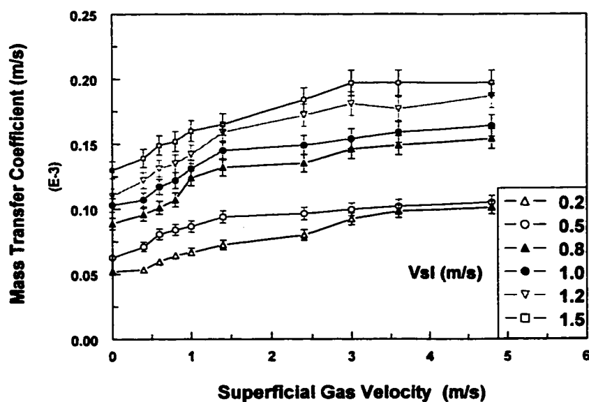
Figure 4.3.2.3 Effect of superficial gas velocity on the average mass transfer coefficient in slug flow and other flows with 20% input oil
