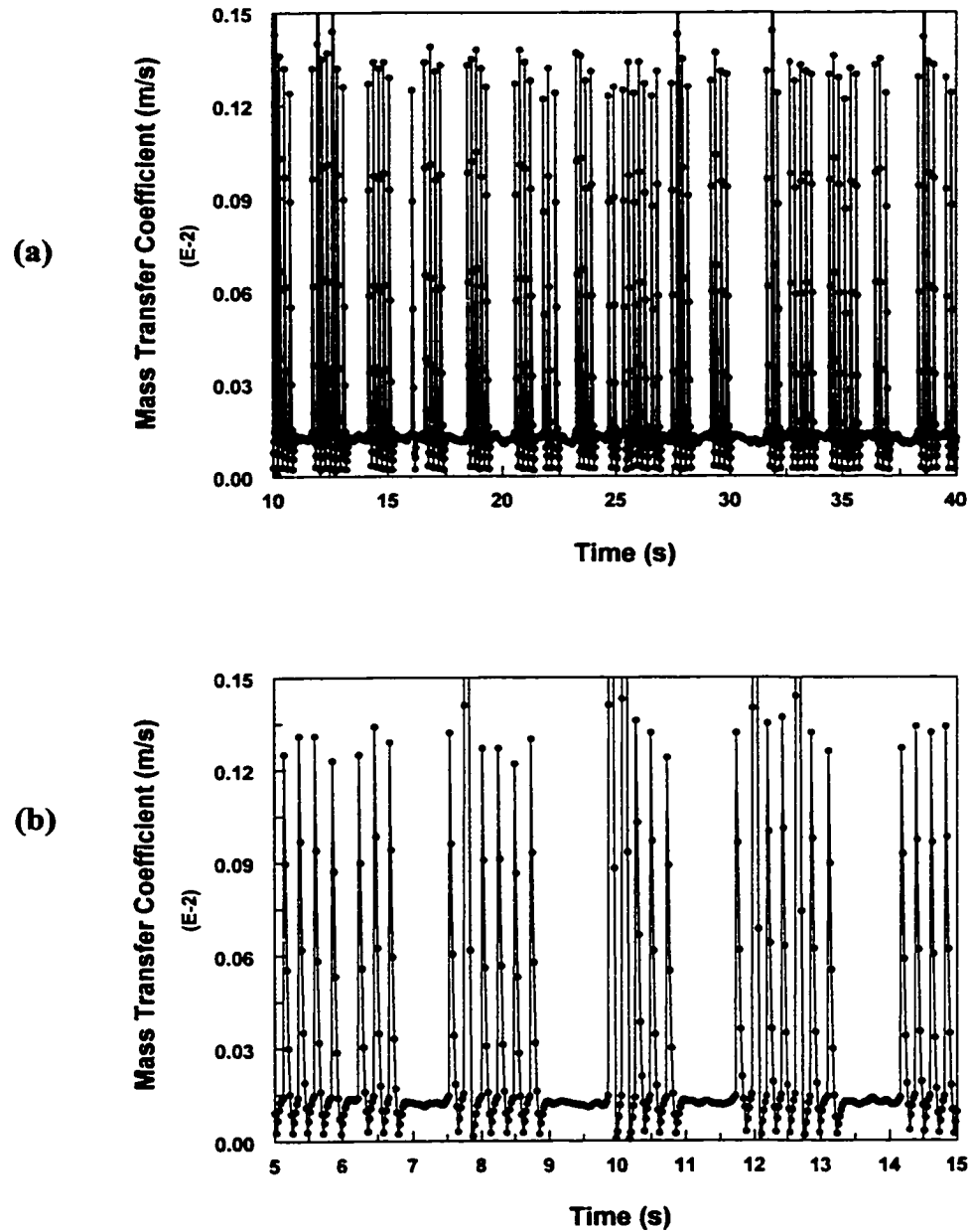
Figure 5.5.3 Instantaneous mass transfer coefficient at V_{sl}=1.0 m/s and V_{sg}=1.4 m/s in water/oil/gas slug flow with 20% input oil (a) 10 – 40 s (b) 5 – 15 s
