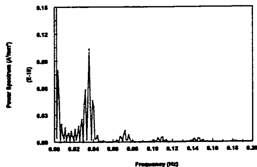
Figure 4.1.4 Power spectrum of the instantaneous limiting current density at 0.03 Hz bubble in the electrochemical cell
