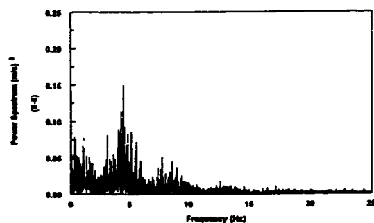
Figure 4.3.15-i Power spectrum of the instantaneous mass transfer coefficient at V_{sl}=1.2 m/s and V_{sg}=3.6 m/s in water/gas flow
