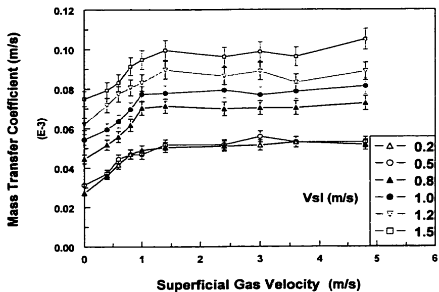
Figure 4.3.1.3 Effect of superficial gas velocity on the average mass transfer coefficient in slug flow and other flows
