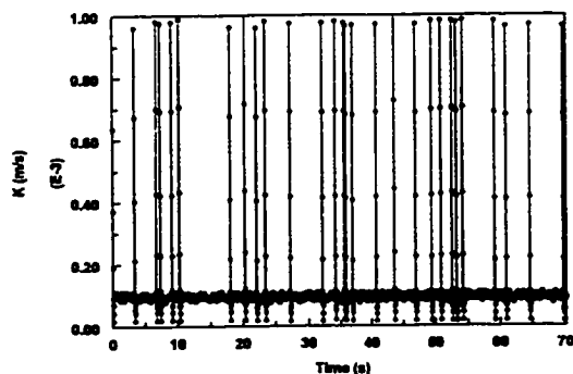
Figure 4.3.1.10-f Instantaneous mass transfer coefficient at V_{sl}=1.5 m/s and V_{sg}=1.4 m/s in water/gas flow
