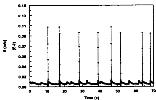
Figure 4.3.1.5-h Instantaneous mass transfer coefficient at V_{sl}=0.2 m/s and V_{sg}=3.0 m/s in water/gas flow
