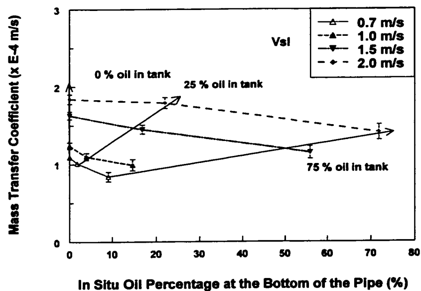
Figure 4.2.5 Average mass transfer coefficient vs in situ oil percentage in full pipe flow
