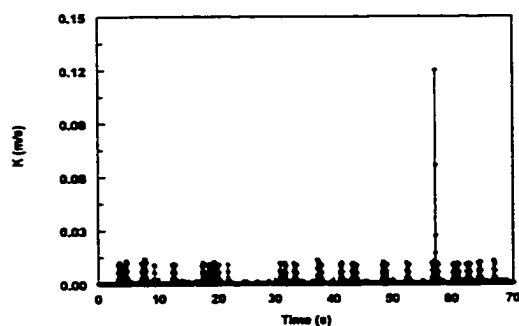
Figure 4.3.2.7-h Instantaneous mass transfer coefficient at V_{sl}=1.0 m/s and V_{sg}=3.0 m/s in water/gas/oil flow with 20% oil
