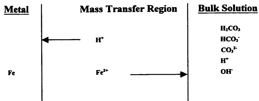
Figure 2.9 Transfer of ions between the metal surface and the bulk solution
