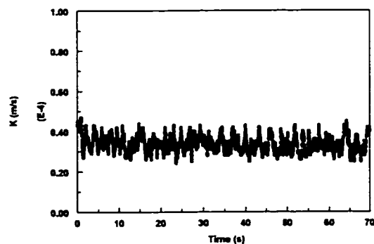
Figure 4.3.1.6-b Instantaneous mass transfer coefficient at V_{sl}=0.5 m/s and V_{sg}=0.4 m/s in water/gas flow
