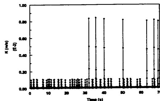
Figure 4.3.1.8-i Instantaneous mass transfer coefficient at V_{sl}=1.0 m/s and V_{sg}=3.6 m/s in water/gas flow
