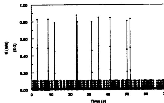
Figure 4.3.1.10-j Instantaneous mass transfer coefficient at V_{sl}=1.5 m/s and V_{sg}=4.8 m/s in water/gas flow
