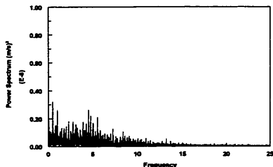
Figure 4.3.1.14-i Power spectrum of the instantaneous mass transfer coefficient at V_{sl}=1.0 m/s and V_{sg}=3.6 m/s in water/gas flow
