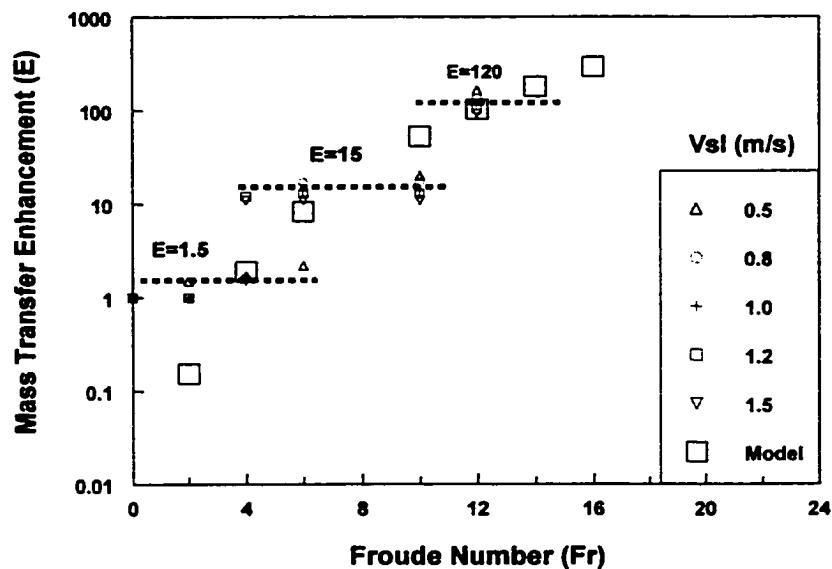
Figure 4.4.9 Relationship between mass transfer enhancement and Froude number
