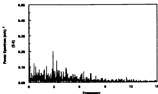
Figure 4.3.1.16-f Power spectrum of the instantaneous mass transfer coefficient at V_{sl}=1.5 m/s and V_{sg}=1.4 m/s in water/gas flow
