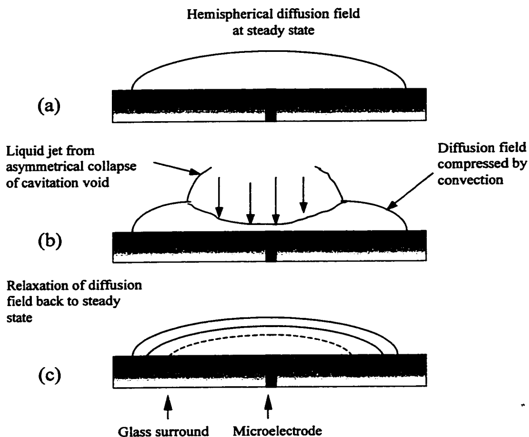
Figure 2.15 Schematic model of the proposed sequence of events, (a) The diffusion field at equilibrium prior to the caviatation event, (b) The impact of a microjet as a result of asymmetric collapse of a cavitation bubble over the electrode surface, (c) The relaxation of the diffusion field after the cavitation event is over (Birkin and Silva-Martinez, 1996)
