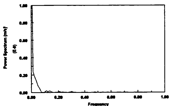
Figure 4.3.12-f Power spectrum of the instantaneous mass transfer coefficient at V_{sl}=0.5 m/s and V_{sg}=1.4 m/s in water/gas flow
