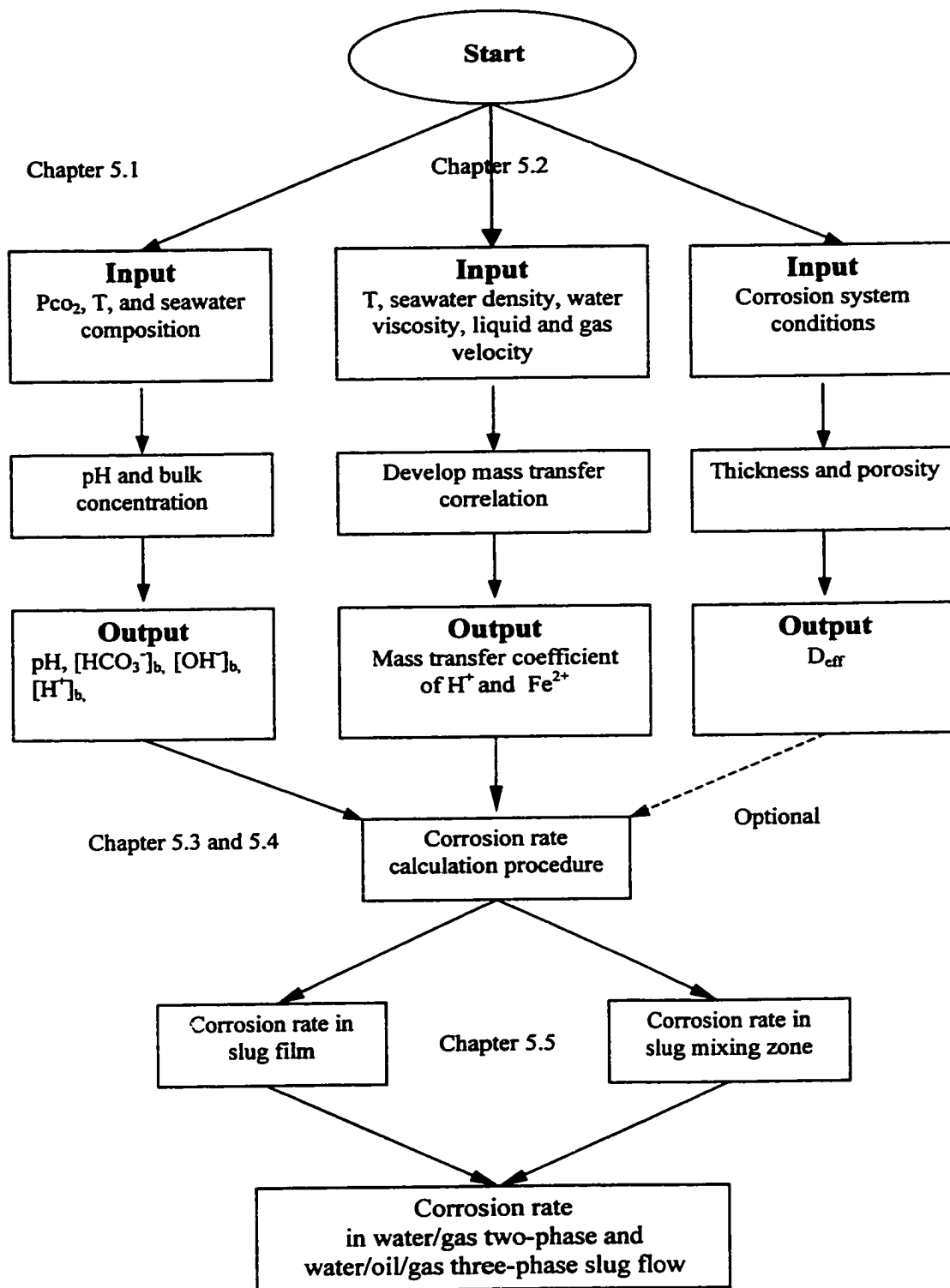
Figure 5.1 Calculation algorithm of corrosion rate in slug flow
