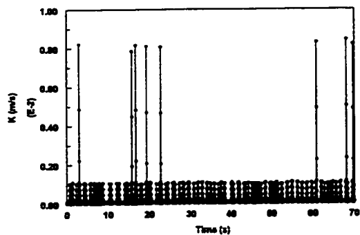
Figure 4.3.1.10-g Instantaneous mass transfer coefficient at V_{sl}=1.5 m/s and V_{sg}=2.4 m/s in water/gas flow
