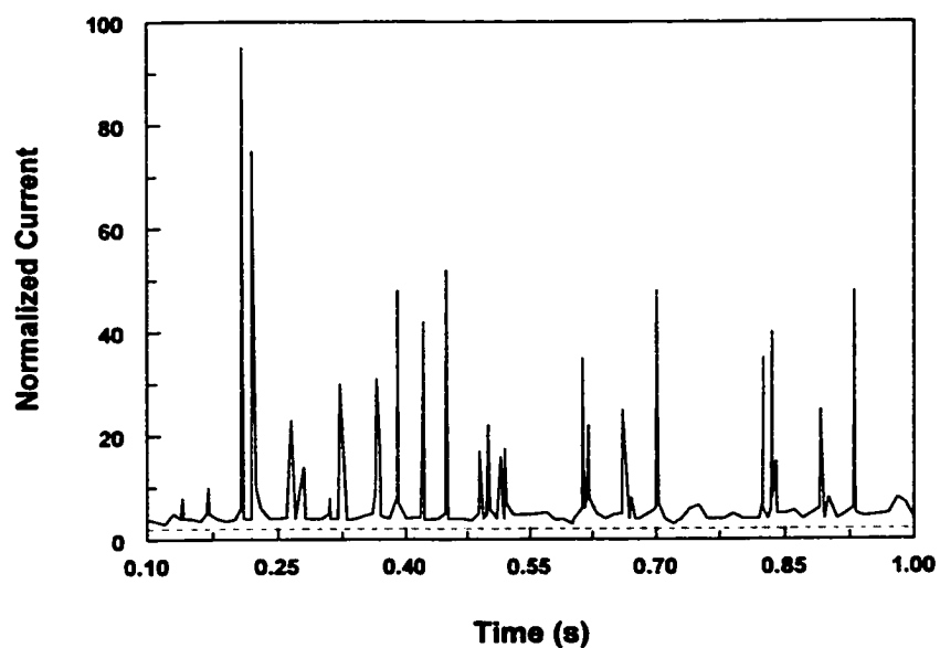
Figure 2.13 Normalized current recorded at a 25 \mu\text{m} diameter Au microelectrode exposed to ultrasound (Birkin and Silva-Martinez, 1996)
