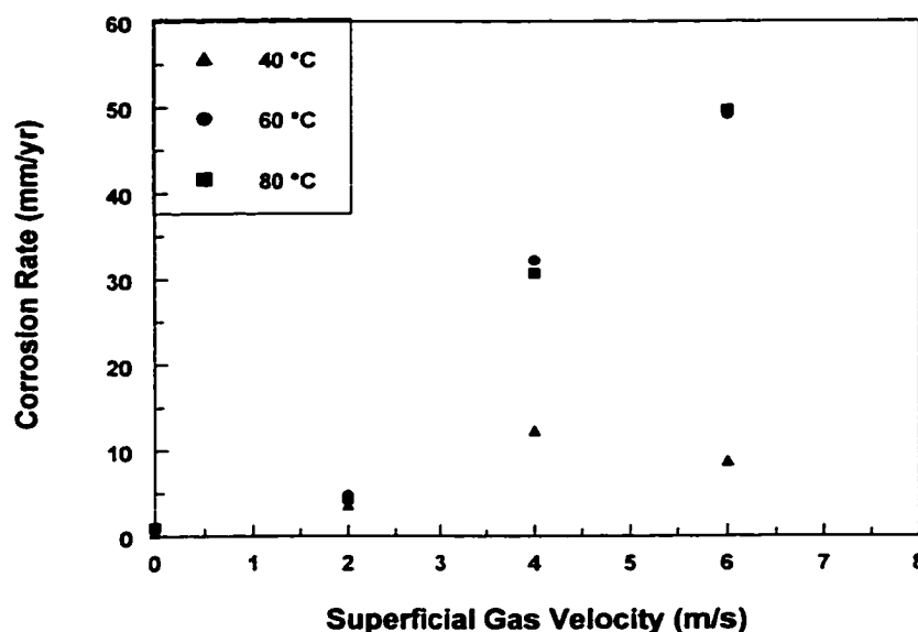
Figure 6.6.1 Predicted corrosion rate vs superficial gas velocity for 40, 60, and 80 °C in ASTM seawater/gas slug flow at 0.27 MPa
