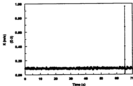
Figure 4.3.1.9-f Instantaneous mass transfer coefficient at V_{sl}=1.2 m/s and V_{sg}=1.4 m/s in water/gas flow
