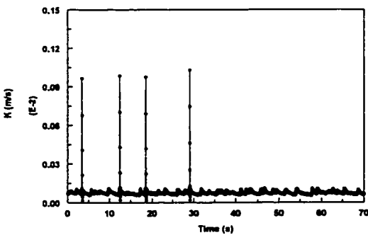
Figure 4.3.1.7-g Instantaneous mass transfer coefficient at V_{sl}=0.8 m/s and V_{sg}=2.4 m/s in water/gas flow
