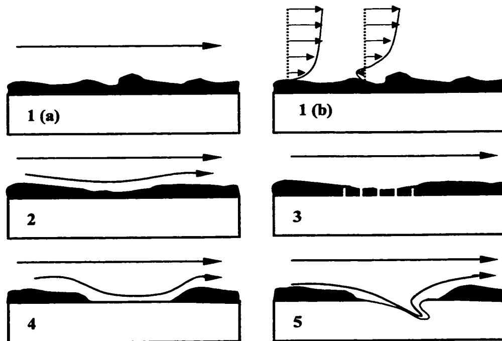
Figure 2.3 Development of flow induced localized corrosion (FILC) mechanism (Schmitt et al. 1999)
