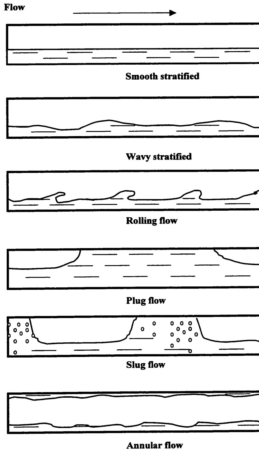
Figure 1.1 Gas/liquid two-phase flow patterns
