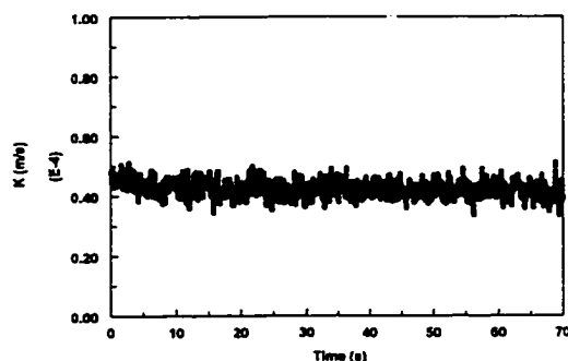
Figure 4.3.1.7-a Instantaneous mass transfer coefficient at V_{sl}=0.8 m/s and V_{sg}=0 m/s in water/gas flow
