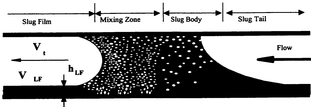
Figure 2.11 Schematic of horizontal slug flow
