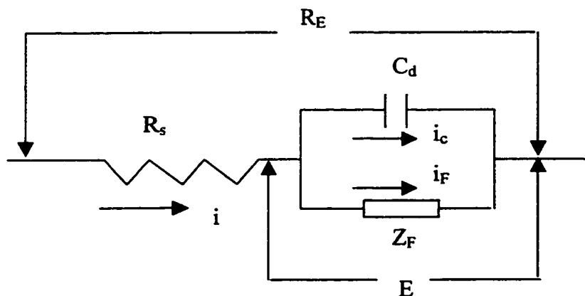
Figure 4.1.19 Schematic of circuit for mass transfer enhancement mechanism by gas bubble or oil droplet
