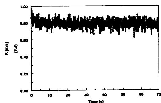
Figure 4.3.1.10-c Instantaneous mass transfer coefficient at V_{sl}=1.5 m/s and V_{sg}=0.6 m/s in water/gas flow
