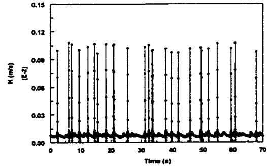
Figure 4.3.1.7-i Instantaneous mass transfer coefficient at V_{sl}=0.8 m/s and V_{sg}=3.6 m/s in water/gas flow
