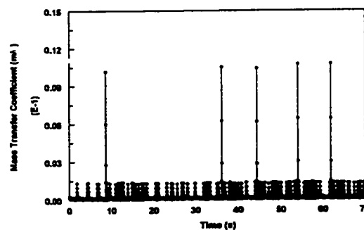
Figure 4.3.3.7-f Instantaneous mass transfer coefficient at V_{sl}=1.0 m/s and V_{sg}=1.4 m/s in water/gas/oil three-phase flow with 40% oil
