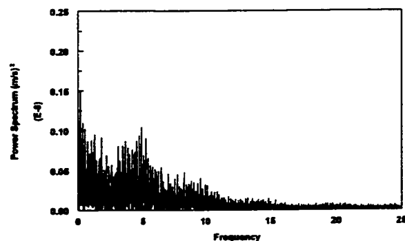
Figure 4.3.12-j Power spectrum of the instantaneous mass transfer coefficient at V_{sl}=0.5 m/s and V_{sg}=4.8 m/s in water/gas flow
