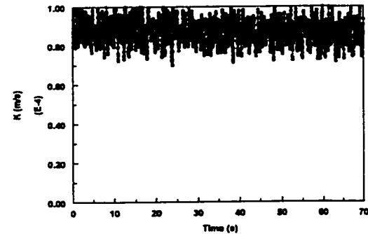
Figure 4.3.1.10-d Instantaneous mass transfer coefficient at V_{sl}=1.5 m/s and V_{sg}=0.8 m/s in water/gas flow
