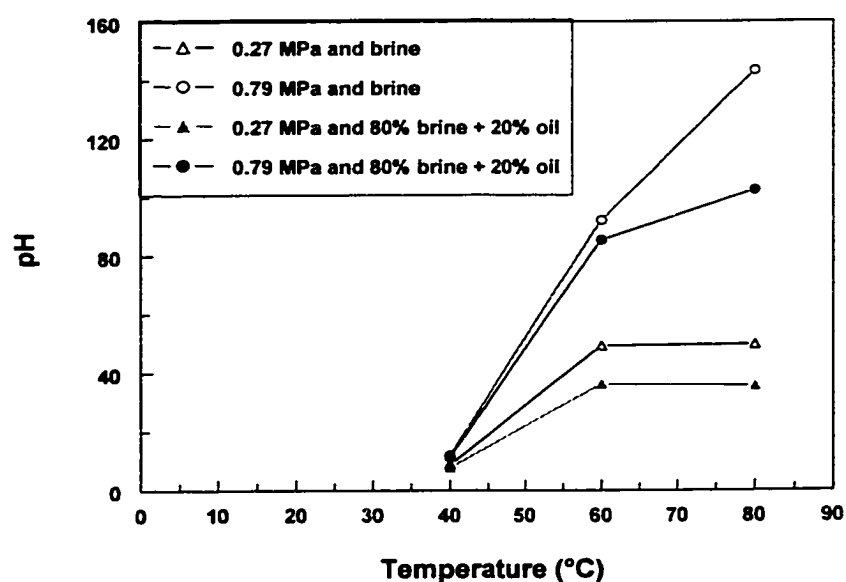
Figure 6.4.1 Influence of temperature on corrosion rates in multiphase slug flow
