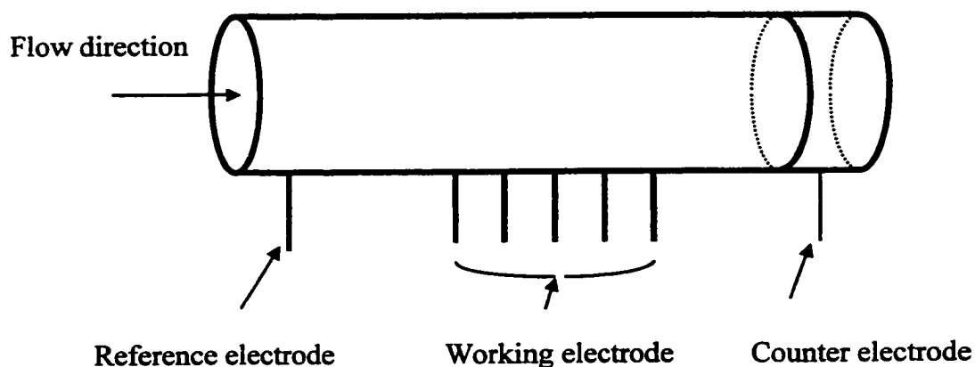
Figure 3.2 Test section used for mass transfer measurement in multiphase flow
