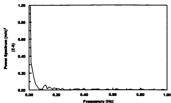
Figure 4.3.11-g Power spectrum of the instantaneous mass transfer coefficient at V_{sl}=0.2 m/s, V_{sg}=2.4 m/s in water/gas flow
