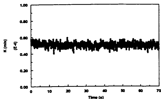
Figure 4.3.1.8-a Instantaneous mass transfer coefficient at V_{sl}=1.0 m/s and V_{sg}=0 m/s in water/gas flow
