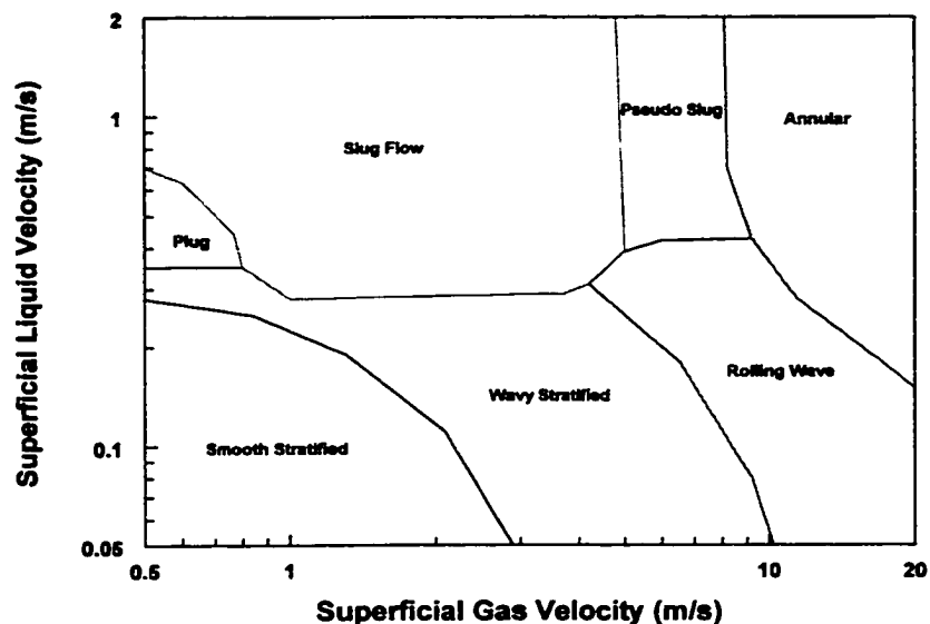
Figure 2.4 A typical flow regime map for gas/liquid two-phase flow in horizontal pipes (Lee, 1993)
