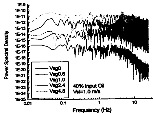
Figure 4.3.3.9 Comparison of p.s.d. at different superficial gas velocities and 1.0 m/s superficial liquid velocity with 40% input oil
