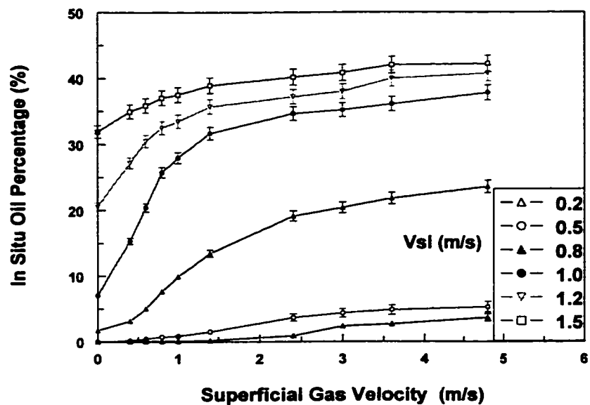
Figure 4.3.3.5 Effect of superficial gas velocity on the in situ oil percentage at the bottom of pipe in water/gas/oil three-phase flow with 40% input oil
