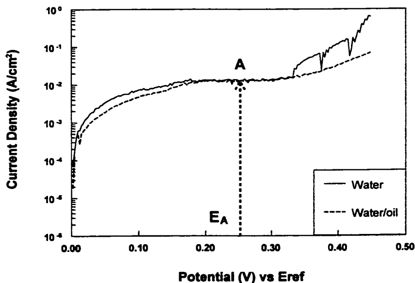
Figure 4.2.8 Limiting current density in water and water/oil flow at velocity 1 m/s. Point A is in the middle of the limiting current plateau. E_A (0.25V) is the applied potential in the potentiostatic experiments
