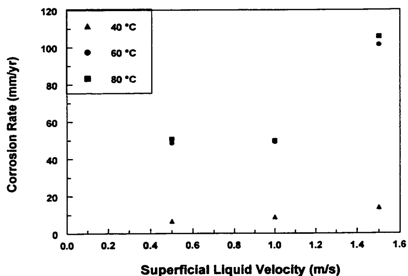
Figure 6.6.2 Predicted corrosion rate vs superficial liquid velocity for 40, 60, and 80 °C in ASTM seawater/gas slug flow at 0.27 MPa
