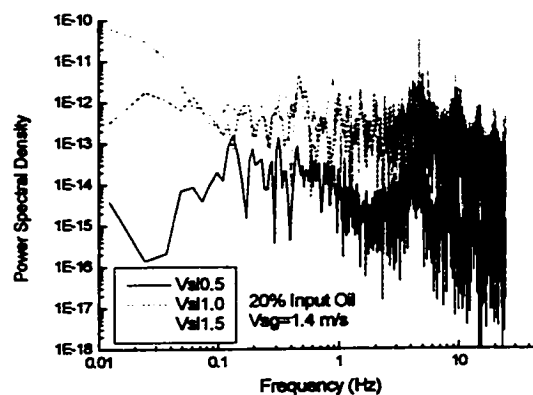
Figure 4.3.3.11 Comparison of p.s.d. at different superficial liquid velocities and 1.4 m/s superficial gas velocity with 20% input oil
