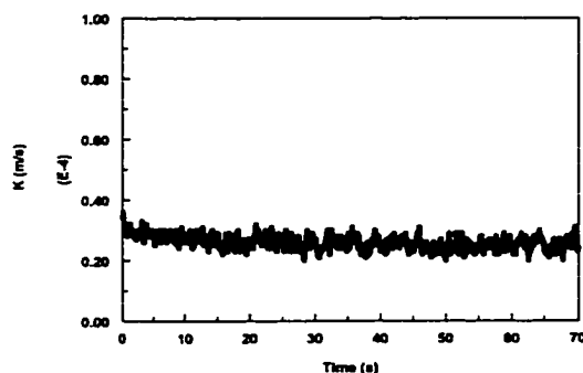
Figure 4.3.1.5-a Instantaneous mass transfer coefficient at V_{sl}=0.2 m/s and V_{sg}=0 m/s in water/gas flow
