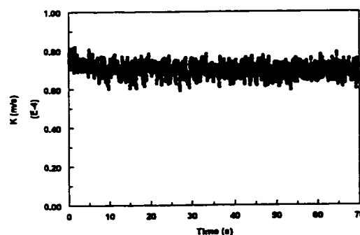
Figure 4.3.1.10-a Instantaneous mass transfer coefficient at V_{sl}=1.5 m/s and V_{sg}=0 m/s in water/gas flow
