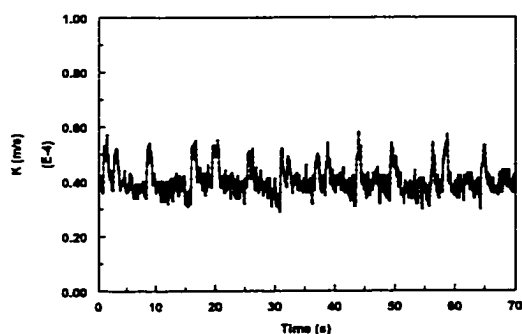
Figure 4.3.1.5-c Instantaneous mass transfer coefficient at V_{sl}=0.2 m/s and V_{sg}=0.6 m/s in water/gas flow
