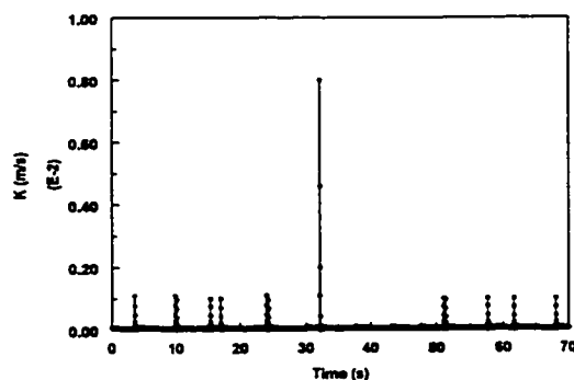
Figure 4.3.1.5-i Instantaneous mass transfer coefficient at V_{sl}=0.2 m/s and V_{sg}=3.6 m/s in water/gas flow
