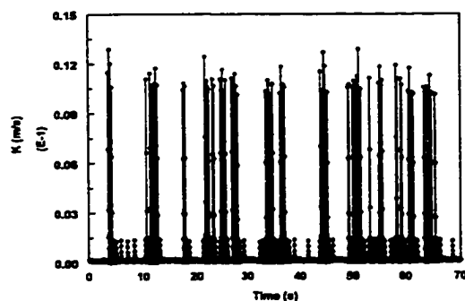
Figure 4.3.2.7-g Instantaneous mass transfer coefficient at V_{sl}=1.0 m/s and V_{sg}=2.4 m/s in water/gas/oil flow with 20% oil
