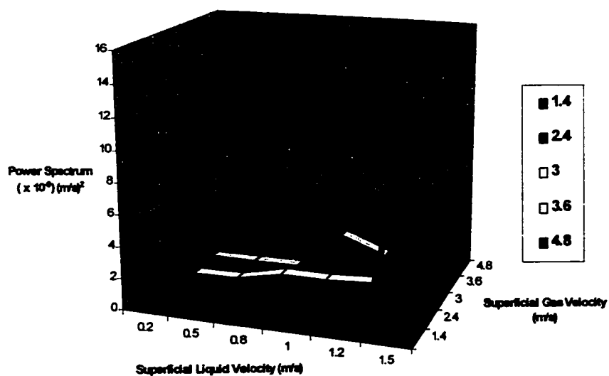
Figure 4.3.1.18 Power spectrum of the instantaneous mass transfer coefficients in different slug flows
