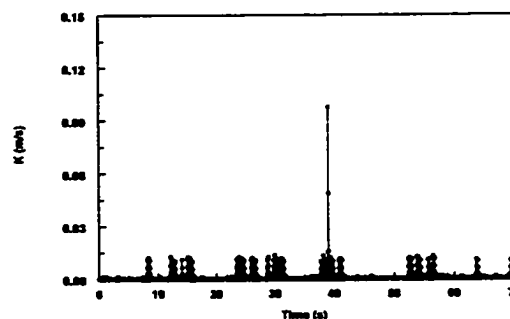
Figure 4.3.2.7-i Instantaneous mass transfer coefficient at V_{sl}=1.0 m/s and V_{sg}=3.6 m/s in water/gas/oil flow with 20% oil
