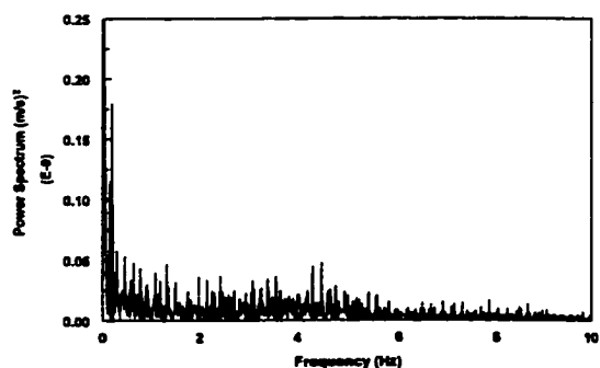
Figure 4.3.11-h Power spectrum of the instantaneous mass transfer coefficient at V_{sl}=0.2 m/s, V_{sg}=3.0 m/s in water/gas flow
