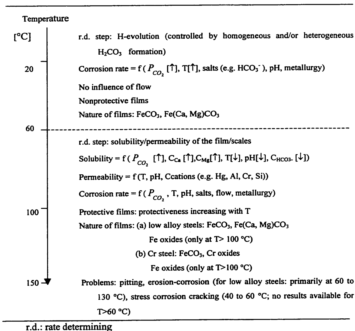
Figure 2.1 Schematic of CO 2 corrosion of carbon steel (Schmitt, 1984a)
