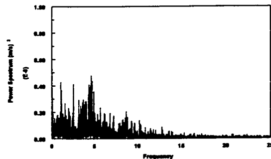
Figure 4.3.1.16-i Power spectrum of the instantaneous mass transfer coefficient at V_{sl}=1.5 m/s and V_{sg}=3.6 m/s in water/gas flow
