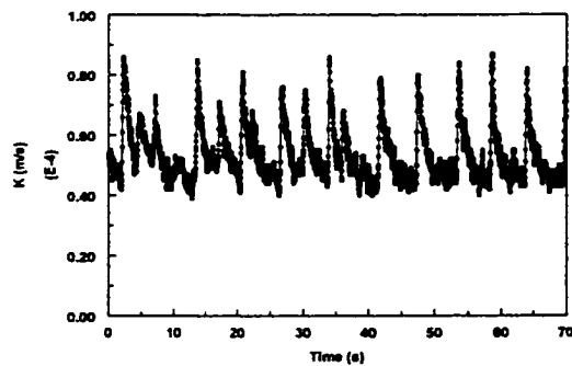
Figure 4.3.1.5-f Instantaneous mass transfer coefficient at V_{sl}=0.2 m/s and V_{sg}=1.4 m/s in water/gas flow
