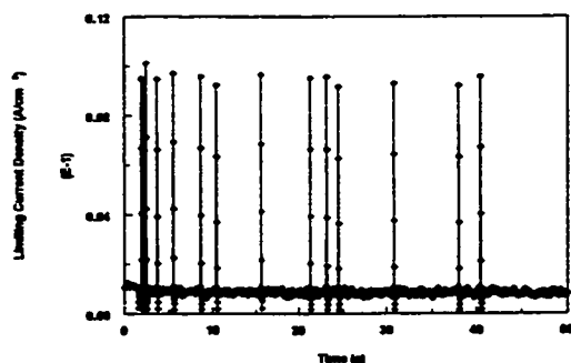
Figure 4.1.5 Instantaneous limiting current density in stationary slug with Froude 4
