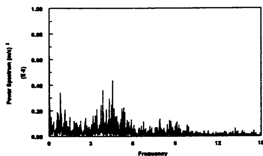
Figure 4.3.1.16-g Power spectrum of the instantaneous mass transfer coefficient at V_{sl}=1.5 m/s and V_{sg}=2.4 m/s in water/gas flow
