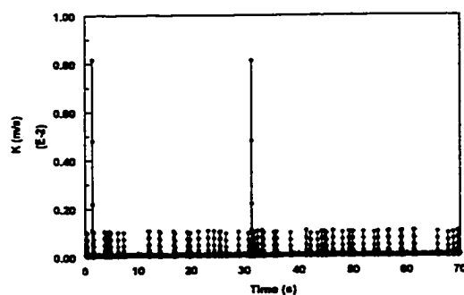
Figure 4.3.1.8-h Instantaneous mass transfer coefficient at V_{sl}=1.0 m/s and V_{sg}=3.0 m/s in water/gas flow
