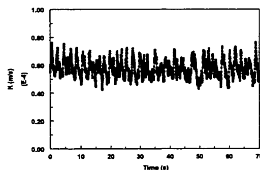
Figure 4.3.1.7-c Instantaneous mass transfer coefficient at V_{sl}=0.8 m/s and V_{sg}=0.6 m/s in water/gas flow
