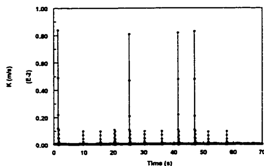
Figure 4.3.1.5-j Instantaneous mass transfer coefficient at V_{sl}=0.2 m/s and V_{sg}=4.8 m/s in water/gas flow
