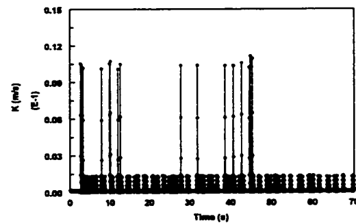
Figure 4.3.2.7-f Instantaneous mass transfer coefficient at V_{sl}=1.0 m/s and V_{sg}=1.4 m/s in water/gas/oil flow with 20% oil
