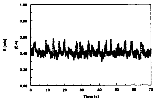
Figure 4.3.1.6-c Instantaneous mass transfer coefficient at V_{sl}=0.5 m/s and V_{sg}=0.6 m/s in water/gas flow
