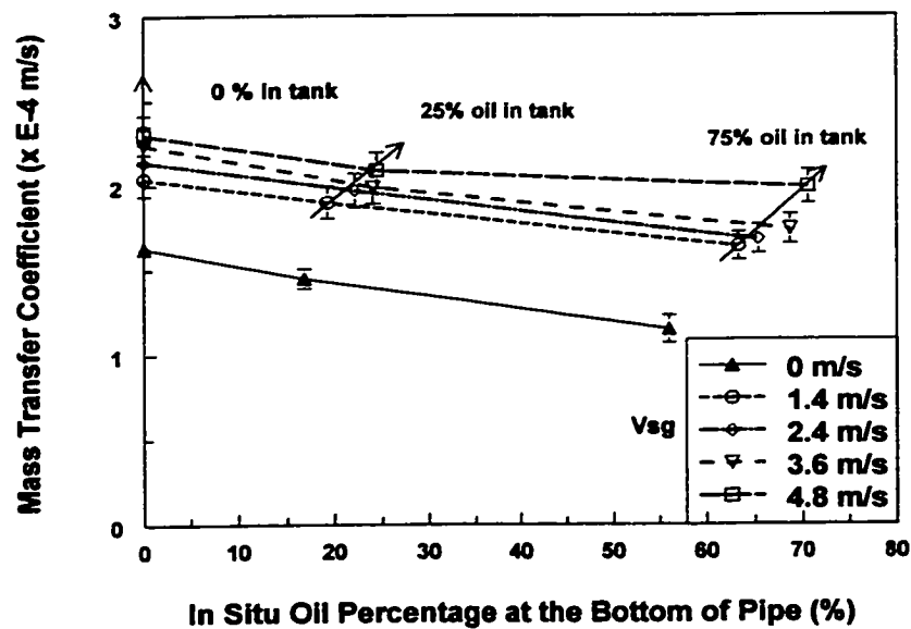
Figure 4.2.7 Comparison of average mass transfer in slug flow and full pipe flow at 1.5 m/s liquid velocity
