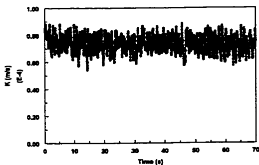
Figure 4.3.1.9-d Instantaneous mass transfer coefficient at V_{sl}=1.2 m/s and V_{sg}=0.8 m/s in water/gas flow
