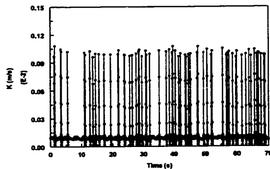
Figure 4.3.1.9-g Instantaneous mass transfer coefficient at V_{sl}=1.2 m/s and V_{sg}=2.4 m/s in water/gas flow
