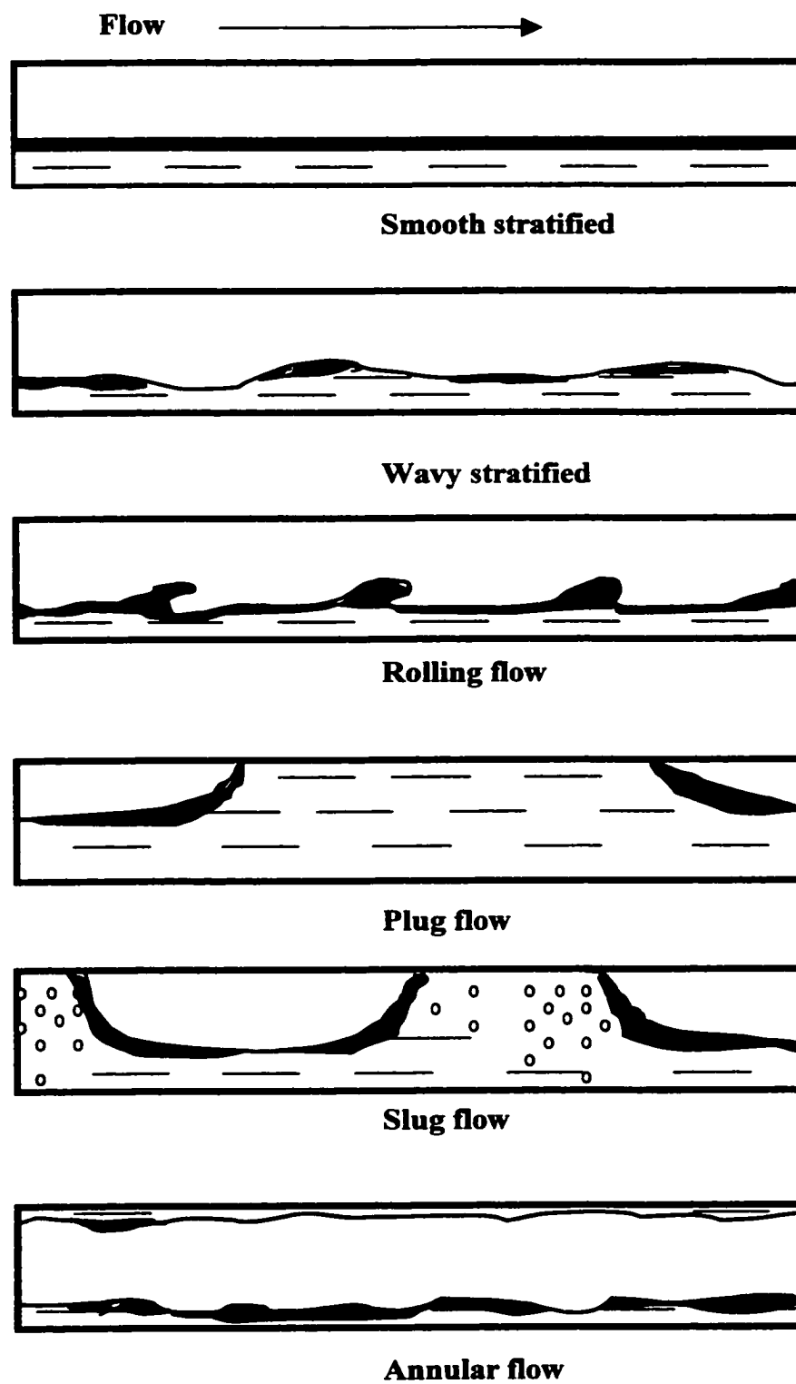
Figure 1.2 Gas/oil/liquid three-phase flow patterns
