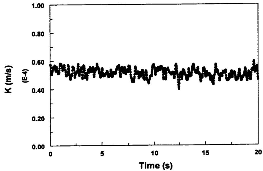
Figure 4.4.3 Instantaneous mass transfer coefficient in water full pipe flow with V_{sl}=1.0 m/s
