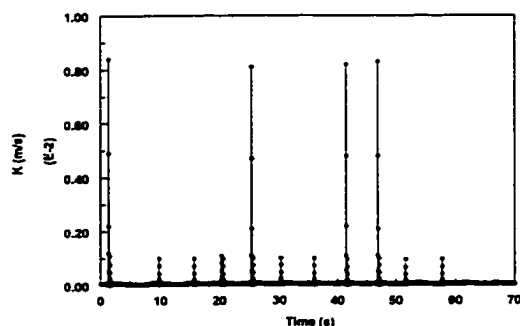
Figure 4.3.1.6-j Instantaneous mass transfer coefficient at V_{sl}=0.5 m/s and V_{sg}=4.8 m/s in water/gas flow
