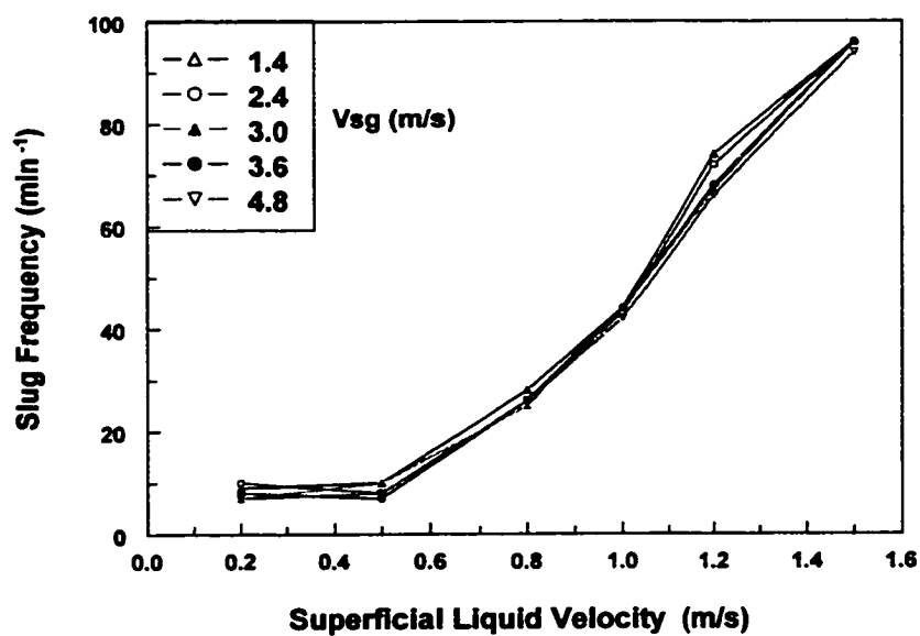
Figure 4.3.3.2 Effect of superficial liquid velocity on the slug frequency with 40% input oil
