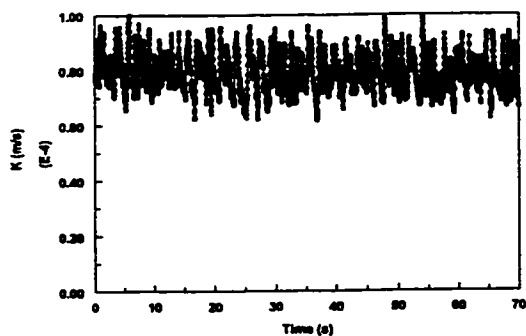
Figure 4.3.1.9-e Instantaneous mass transfer coefficient at V_{sl}=1.2 m/s and V_{sg}=1.0 m/s in water/gas flow
