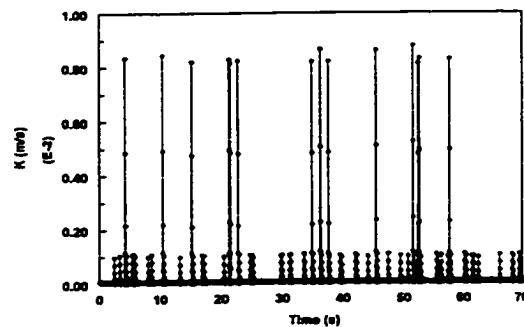
Figure 4.3.1.8-j Instantaneous mass transfer coefficient at V_{sl}=1.0 m/s and V_{sg}=4.8 m/s in water/gas flow
