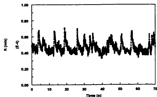
Figure 4.3.1.6-d Instantaneous mass transfer coefficient at V_{sl}=0.5 m/s and V_{sg}=0.8 m/s in water/gas flow
