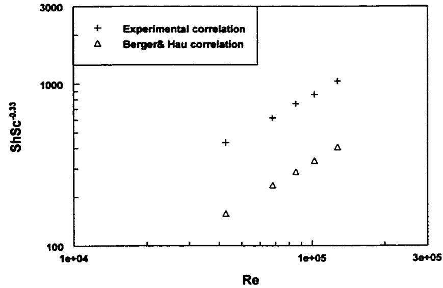
Figure 4.4.1 Experimental mass transfer correlation and Berger & Hau mass transfer correlation
