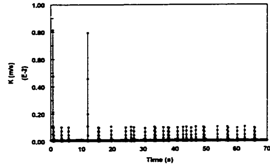
Figure 4.3.1.7-h Instantaneous mass transfer coefficient at V_{sl}=0.8 m/s and V_{sg}=3.0 m/s in water/gas flow
