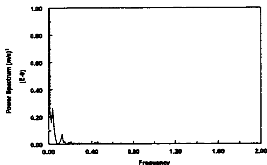
Figure 4.3.12-g Power spectrum of the instantaneous mass transfer coefficient at V_{sl}=0.5 m/s and V_{sg}=2.4 m/s in water/gas flow
