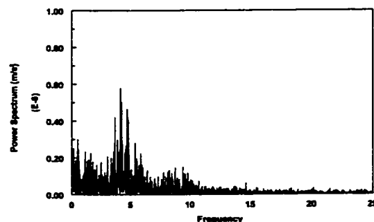
Figure 4.3.1.16-j Power spectrum of the instantaneous mass transfer coefficient at V_{sl}=1.5 m/s and V_{sg}=4.8 m/s in water/gas flow
