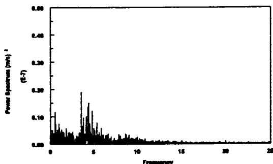
Figure 4.3.1.16-h Power spectrum of the instantaneous mass transfer coefficient at V_{sl}=1.5 m/s and V_{sg}=3.0 m/s in water/gas flow
