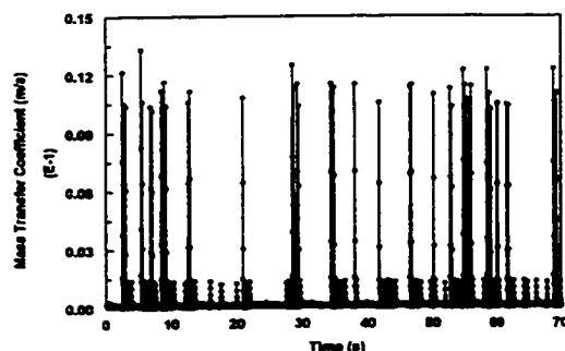
Figure 4.3.3.7-h Instantaneous mass transfer coefficient at V_{sl}=1.0 m/s and V_{sg}=3.0 m/s in water/gas/oil three-phase flow with 40% oil
