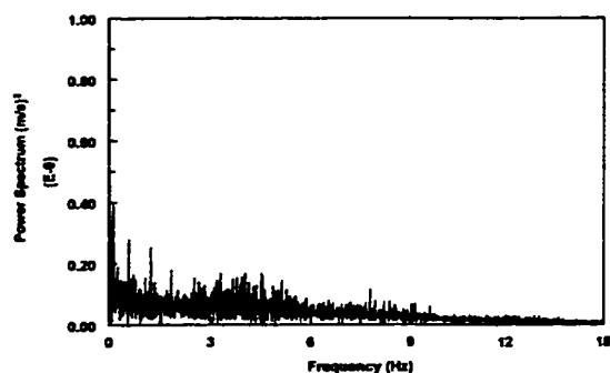
Figure 4.3.11-i Power spectrum of the instantaneous mass transfer coefficient at V_{sl}=0.2 m/s, V_{sg}=3.6 m/s in water/gas flow
