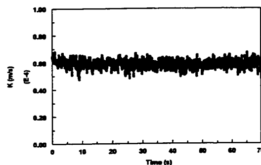
Figure 4.3.1.9-a Instantaneous mass transfer coefficient at V_{sl}=1.2 m/s and V_{sg}=0 m/s in water/gas flow
