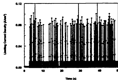
Figure 4.1.8 Instantaneous limiting current density in stationary slug with Froude 7
