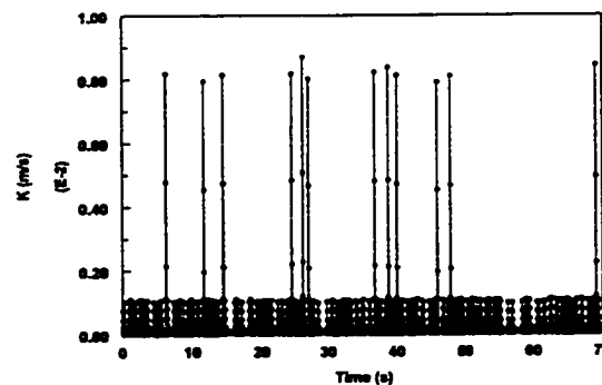
Figure 4.3.1.10-i Instantaneous mass transfer coefficient at V_{sl}=1.5 m/s and V_{sg}=3.6 m/s in water/gas flow
