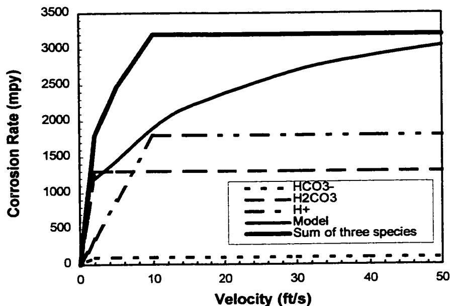
Figure 2.6 Schematic of corrosion concentration of various cathodic reactants and comparison with the model (Dayalan et al. 1995)
