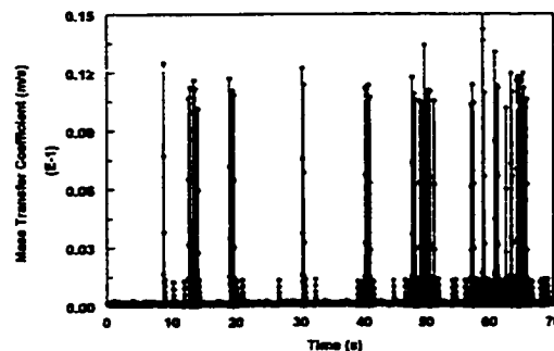
Figure 4.3.3.7-i Instantaneous mass transfer coefficient at V_{sl}=1.0 m/s and V_{sg}=3.6 m/s in water/gas/oil three-phase flow with 40% oil
