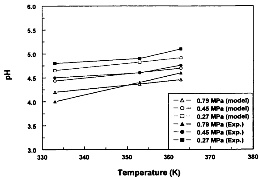
Figure 6.1.2 Comparison of experimental data and predicted pH values for brine
