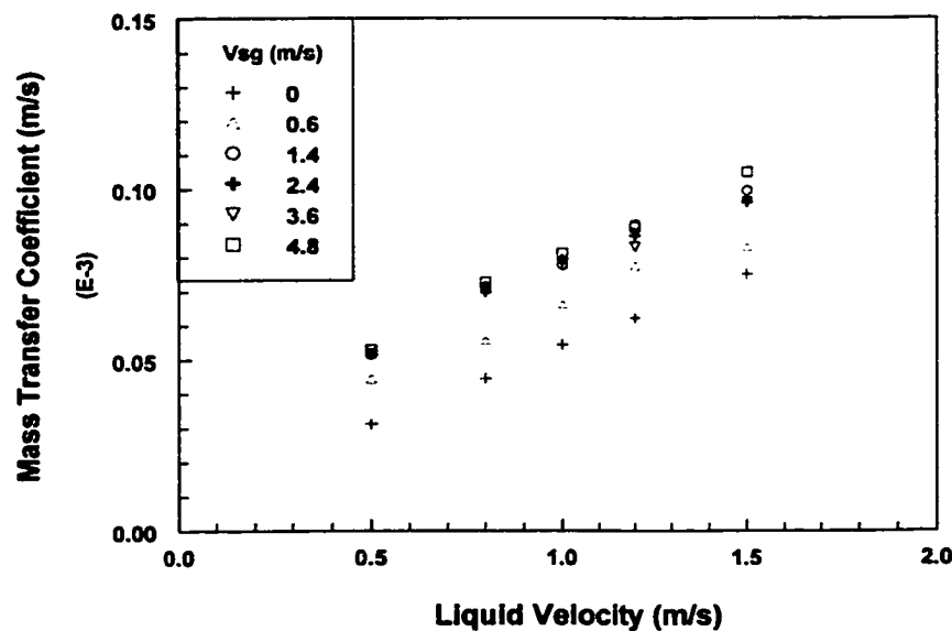
Figure 4.4.2 Average mass transfer measurement in water/gas two-phase flow
