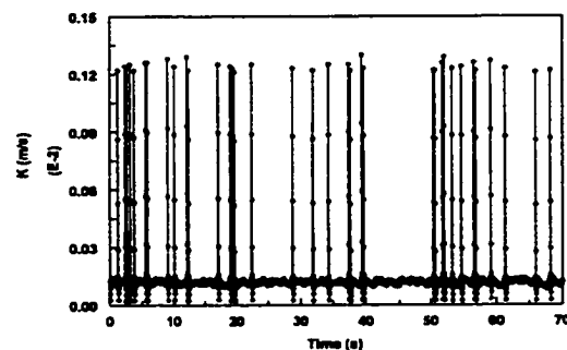
Figure 4.3.2.7-e Instantaneous mass transfer coefficient at V_{sl}=1.0 m/s and V_{sg}=1.0 m/s in water/gas/oil flow with 20% oil
