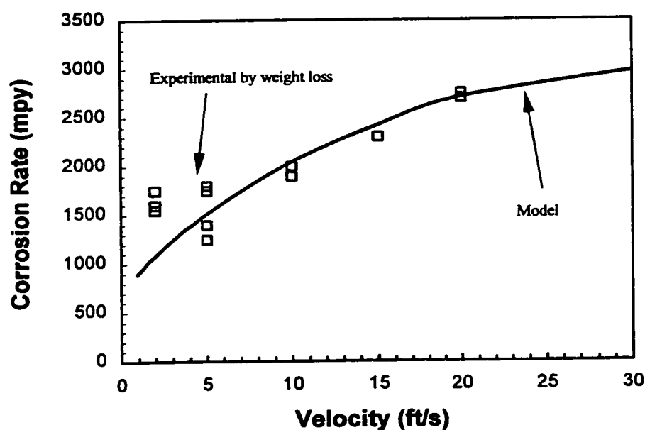
Figure 2.7 Comparison of corrosion rates from model predictions and experiments at 150 psig CO 2 partial pressure, 160 °F, and 3.4 pH as a function of velocity in 1" pipe (Dayalan et al. 1995).
