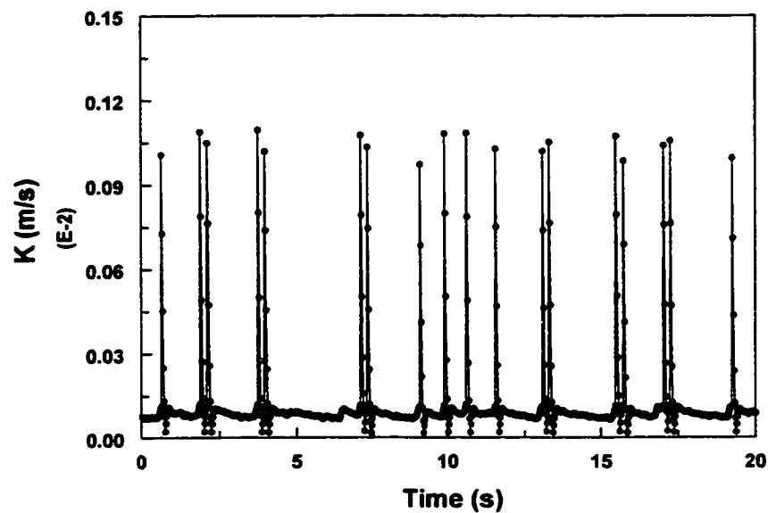
Figure 4.4.7 Instantaneous mass transfer coefficient in water/gas two-phase flow with V_{sl}=1.0 m/s and V_{sg}=3.6 m/s
