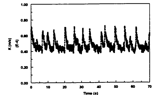
Figure 4.3.1.6-e Instantaneous mass transfer coefficient at V_{sl}=0.5 m/s and V_{sg}=1.0 m/s in water/gas flow
