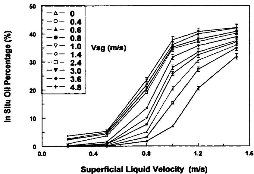
Figure 4.3.3.6 Effect of superficial liquid velocity on the in situ oil percentage at the bottom of pipe in water/gas/oil three-phase flow with 40% input oil
