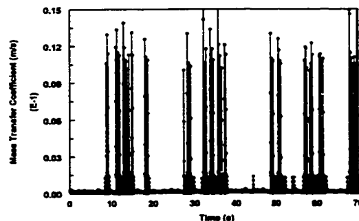
Figure 4.3.3.7-j Instantaneous mass transfer coefficient at V_{sl}=1.0 m/s and V_{sg}=4.8 m/s in water/gas/oil three-phase flow with 40% oil
