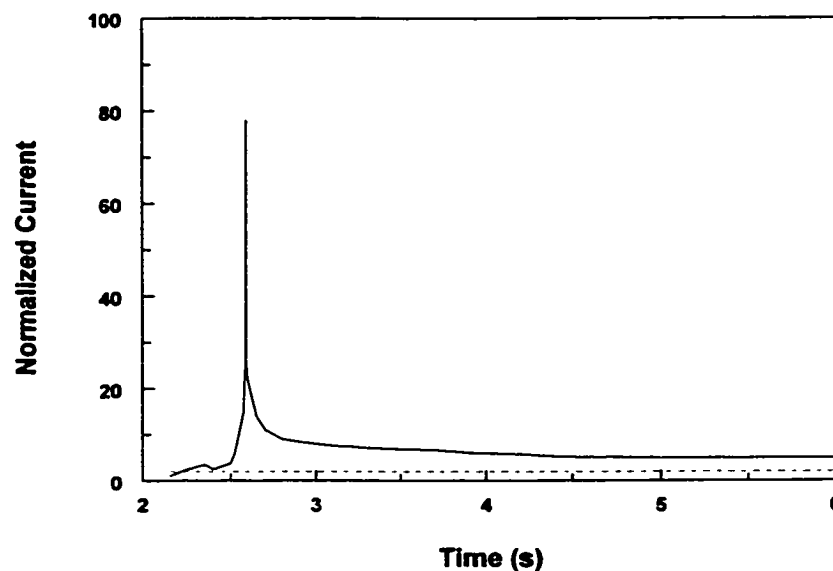
Figure 2.14 A single normalized current-time transient recorded at a 25 \mu\text{m} diameter Au microelectrode exposed to ultrasound (Birkin and Silva-Martinez, 1996)
