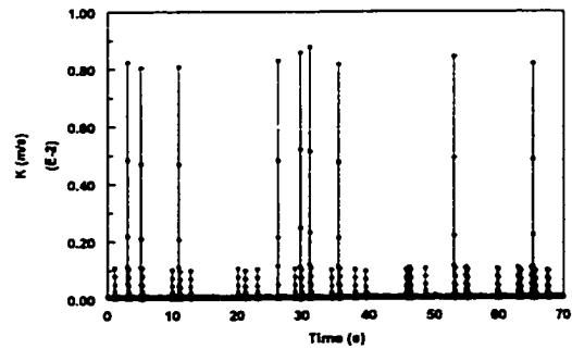
Figure 4.3.1.7-j Instantaneous mass transfer coefficient at V_{sl}=0.8 m/s and V_{sg}=4.8 m/s in water/gas flow
