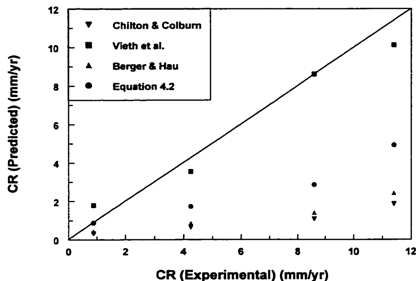
Figure 6.2.1 Predicted vs experimental corrosion rates for brine by using several mass transfer correlations in full pipe flow
