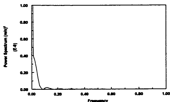
Figure 4.3.1.14-f Power spectrum of the instantaneous mass transfer coefficient at V_{sl}=1.0 m/s and V_{sg}=1.4 m/s in water/gas flow
