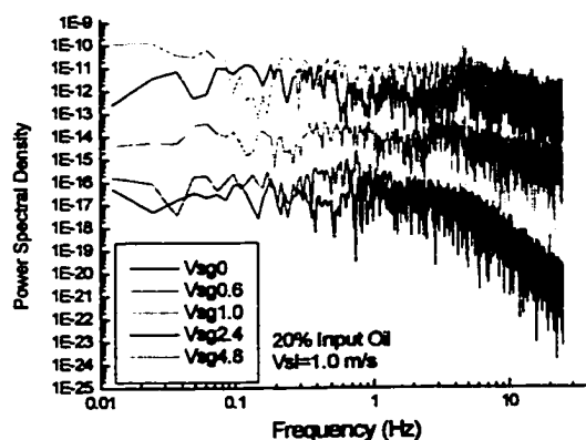
Figure 4.3.3.8 Comparison of p.s.d. at different superficial gas velocities and 1.0 m/s superficial liquid velocity with 20% input oil
