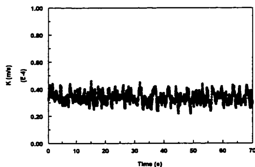
Figure 4.3.1.5-b Instantaneous mass transfer coefficient at V_{sl}=0.2 m/s and V_{sg}=0.4 m/s in water/gas flow
