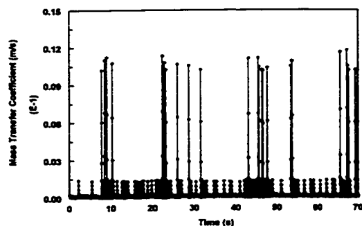
Figure 4.3.3.7-g Instantaneous mass transfer coefficient at V_{sl}=1.0 m/s and V_{sg}=2.4 m/s in water/gas/oil three-phase flow with 40% oil
