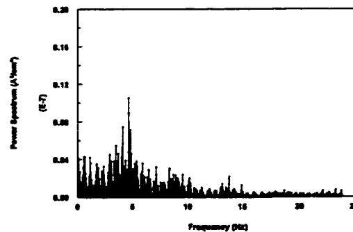
Figure 4.1.10 Power spectrum of the instantaneous limiting current density in stationary slug with Froude 5
