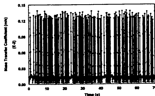
Figure 4.3.3.7-e Instantaneous mass transfer coefficient at V_{sl}=1.0 m/s and V_{sg}=1.0 m/s in water/gas/oil three-phase flow with 40% oil
