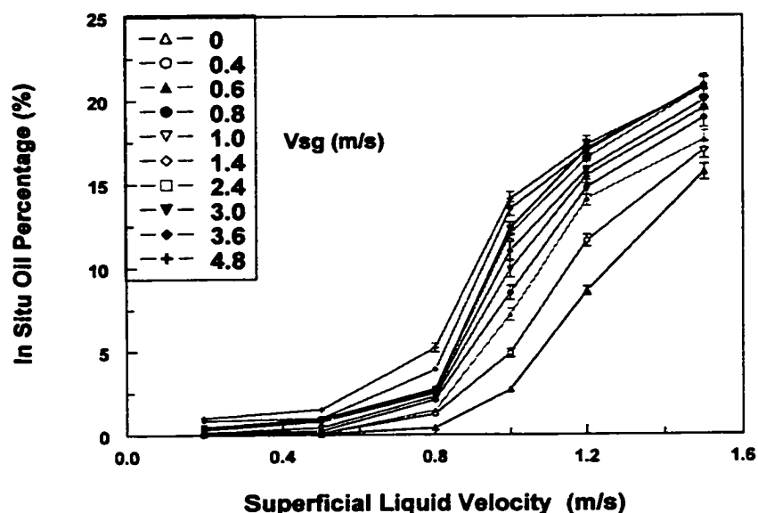
Figure 4.3.2.6 Effect of superficial liquid velocity on the in situ oil percentage at the bottom of pipe in water/gas/oil three-phase flow with 20% input oil
