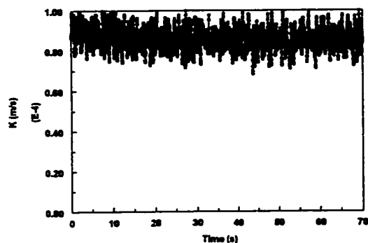
Figure 4.3.1.10-e Instantaneous mass transfer coefficient at V_{sl}=1.5 m/s and V_{sg}=1.0 m/s in water/gas flow
