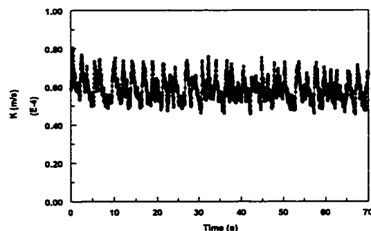
Figure 4.3.1.7-d Instantaneous mass transfer coefficient at V_{sl}=0.8 m/s and V_{sg}=0.8 m/s in water/gas flow
