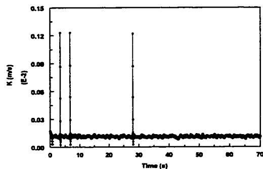
Figure 4.3.2.7-d Instantaneous mass transfer coefficient at V_{sl}=1.0 m/s and V_{sg}=0.8 m/s in water/gas/oil flow with 20% oil
