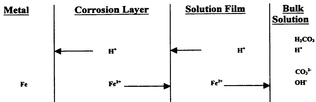
Figure 2.10 Effect of a corrosion product layer on the transfer of ions between the metal surface and the bulk solution
