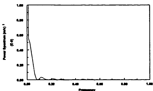
Figure 4.3.15-f Power spectrum of the instantaneous mass transfer coefficient at V_{sl}=1.2 m/s and V_{sg}=1.4 m/s in water/gas flow
