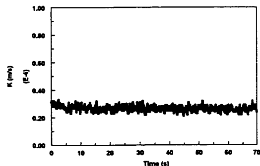
Figure 4.3.1.6-a Instantaneous mass transfer coefficient at V_{sl}=0.5 m/s and V_{sg}=0 m/s in water/gas flow
