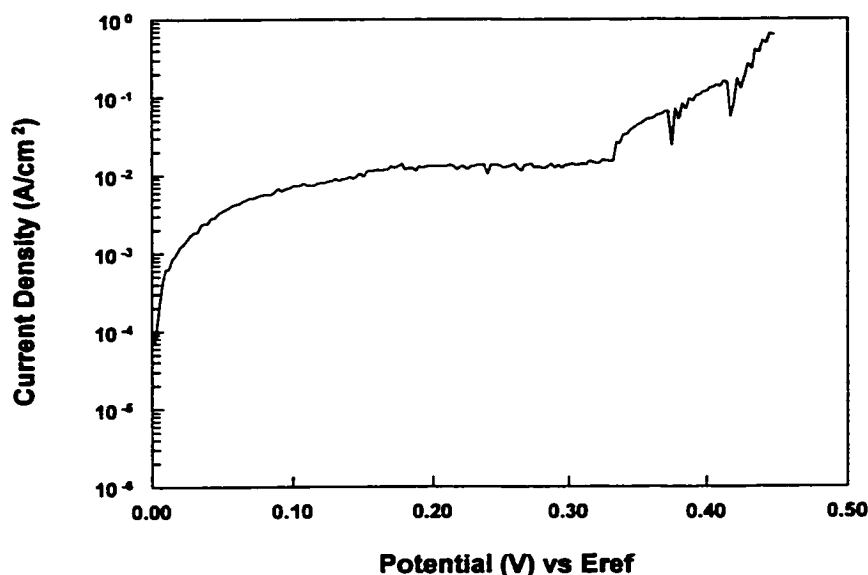
Figure 4.2.1 Limiting current density at liquid velocity of 1 m/s in full pipe flow without oil
