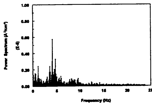
Figure 4.1.18 Power spectrum of the instantaneous limiting current density at slug flow with V_{sl}=1.5 m/s and V_{sg}=4.8 m/s
