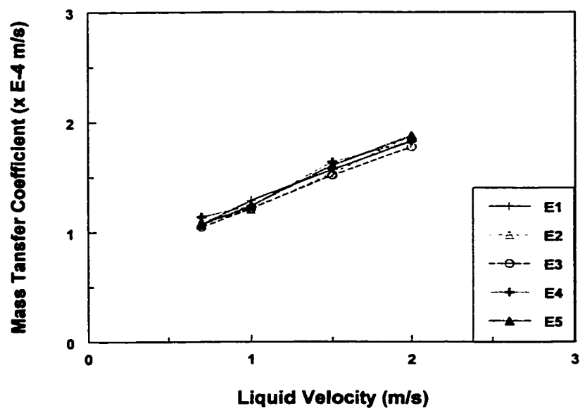
Figure 4.2.2 Local mass transfer coefficient of five electrodes vs liquid velocity in full pipe flow without oil
