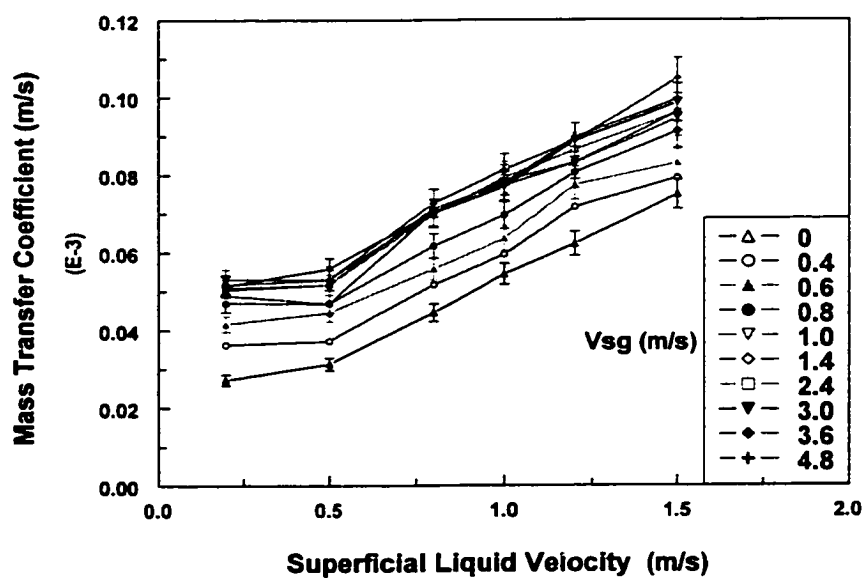
Figure 4.3.1.4 Effect of superficial liquid velocity on the average mass transfer coefficient in slug flow and other flows
