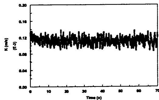
Figure 4.3.2.7-c Instantaneous mass transfer coefficient at V_{sl}=1.0 m/s and V_{sg}=0.6 m/s in water/gas/oil flow with 20% oil
