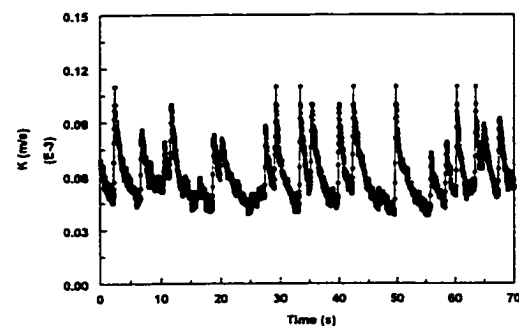
Figure 4.3.1.6-g Instantaneous mass transfer coefficient at V_{sl}=0.5 m/s and V_{sg}=2.4 m/s in water/gas flow
