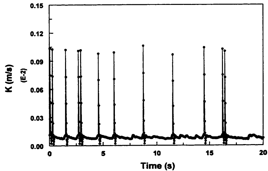
Figure 4.4.6 Instantaneous mass transfer coefficient in water/gas two-phase flow with V_{sl}=1.0 m/s and V_{sg}=2.4 m/s
