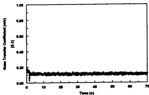
Figure 4.3.3.7-b Instantaneous mass transfer coefficient at V_{sl}=1.0 m/s and V_{sg}=0.4 m/s in water/gas/oil three-phase flow with 40% oil
