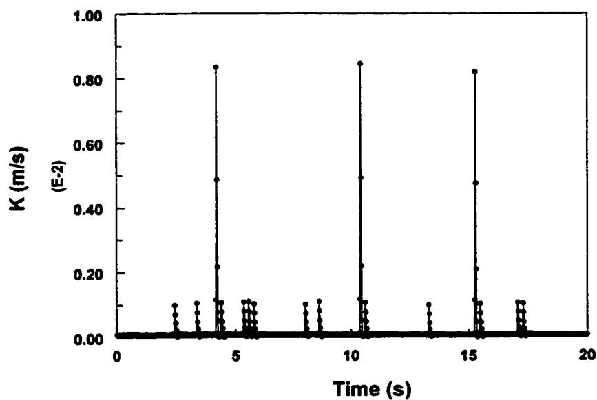
Figure 4.4.8 The Instantaneous mass transfer coefficient in water/gas two-phase flow with V_{sl}=1.0 m/s and V_{sg}=4.8 m/s
