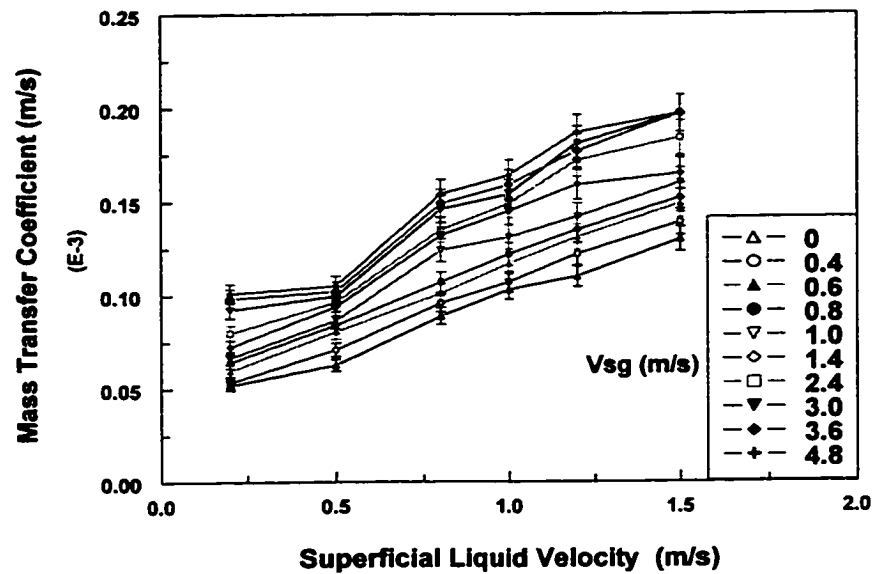
Figure 4.3.2.4 Effect of superficial liquid velocity on the average mass transfer coefficient in slug flow and other flows with 20% input oil
