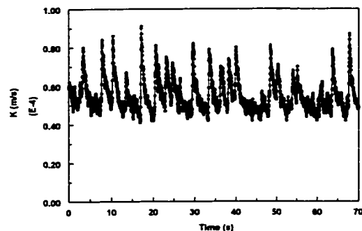
Figure 4.3.1.6-f Instantaneous mass transfer coefficient at V_{sl}=0.5 m/s and V_{sg}=1.4 m/s in water/gas flow
