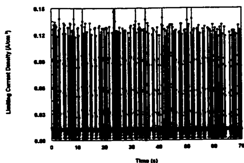
Figure 4.1.15 Instantaneous mass transfer coefficient in slug flow with V_{sl}=1.5 m/s and V_{sg}=4.8 m/s
