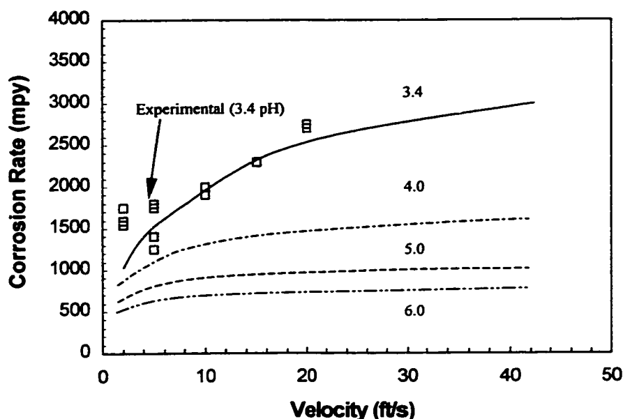
Figure 2.8 Comparison of corrosion rates from model predictions and experiments with E/CRC experimental data at 150 psig CO 2 partial pressure, 160 °F, and 3.4 pH as a function of velocity in 1" pipe (Dayalan et al. 1995).
