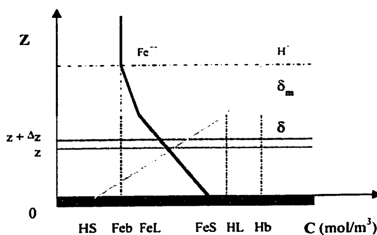
Figure 5.4.1 Schematic of mass transfer with the presence of corrosion product film
