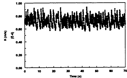
Figure 4.3.1.8-e Instantaneous mass transfer coefficient at V_{sl}=1.0 m/s and V_{sg}=1.0 m/s in water/gas flow
