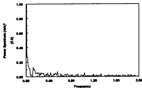
Figure 4.3.12-h Power spectrum of the instantaneous mass transfer coefficient at V_{sl}=0.5 m/s and V_{sg}=3.0 m/s in water/gas flow
