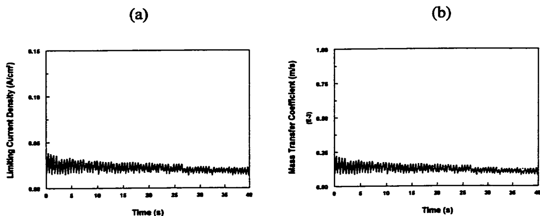
Figure 4.2.9 Instantaneous limiting current density (a) and instantaneous mass transfer coefficient (b) in water flow at velocity 1 m/s
