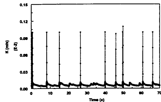
Figure 4.3.1.6-h Instantaneous mass transfer coefficient at V_{sl}=0.5 m/s and V_{sg}=3.0 m/s in water/gas flow
