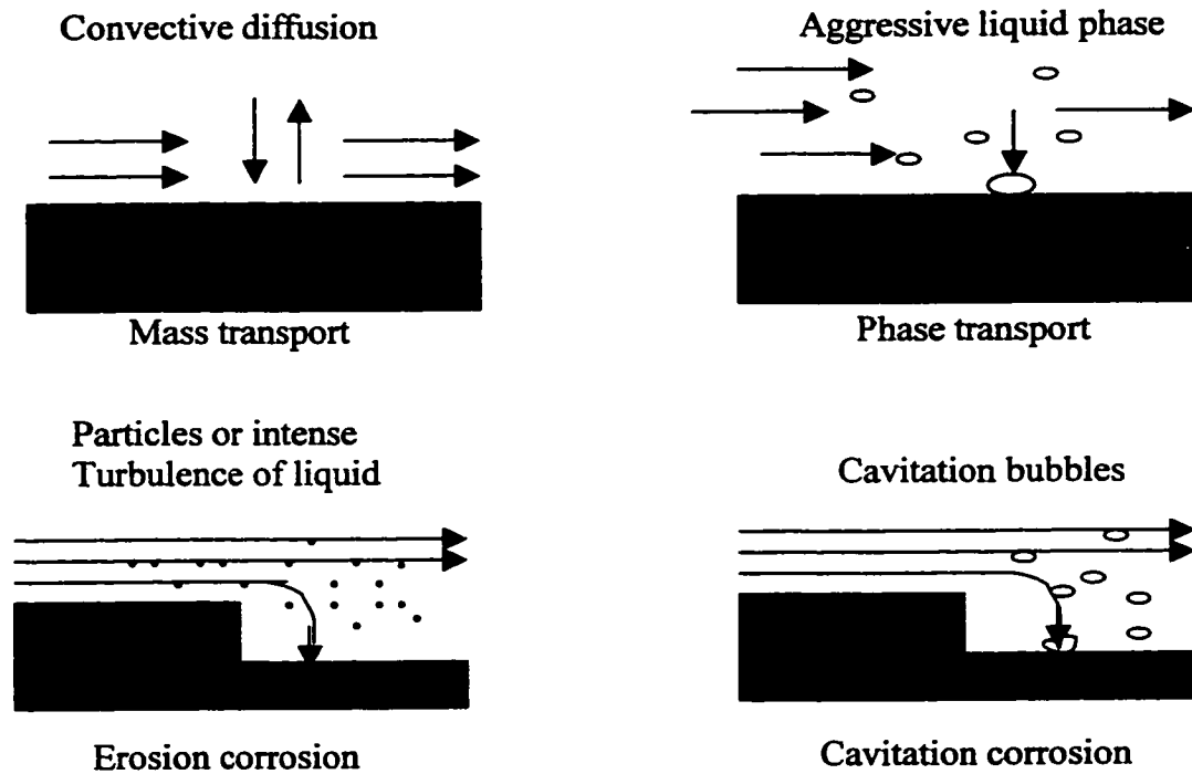
Figure 2.2 Schematic of the four main types of flow-accelerated corrosion (Poulson, 1993)
