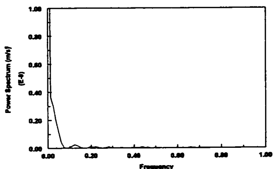
Figure 4.3.13-f Power spectrum of the instantaneous mass transfer coefficient at V_{sl}=0.8 m/s and V_{sg}=1.4 m/s in water/gas flow
