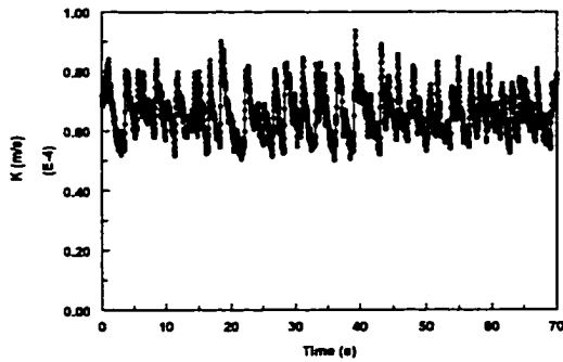
Figure 4.3.1.7-e Instantaneous mass transfer coefficient at V_{sl}=0.8 m/s and V_{sg}=1.0 m/s in water/gas flow
