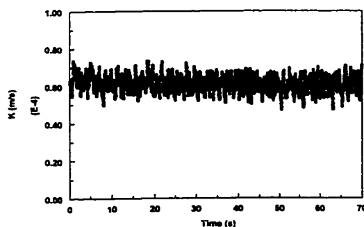
Figure 4.3.1.8-c Instantaneous mass transfer coefficient at V_{sl}=1.0 m/s and V_{sg}=0.6 m/s in water/gas flow
