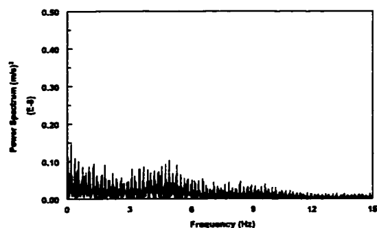
Figure 4.3.11-j Power spectrum of the instantaneous mass transfer coefficient at V_{sl}=0.2 m/s, V_{sg}=4.8 m/s in water/gas flow
