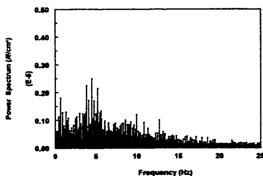
Figure 4.1.11 Power spectrum of the instantaneous limiting current density in stationary slug with Froude 6
