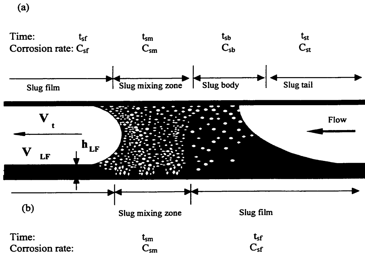
Figure 5.5.2 Calculation of overall corrosion rate by (a) four parts and (b) two parts in slug flow
