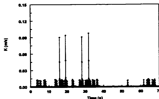
Figure 4.3.2.7-j Instantaneous mass transfer coefficient at V_{sl}=1.0 m/s and V_{sg}=4.8 m/s in water/gas/oil flow with 20% oil
