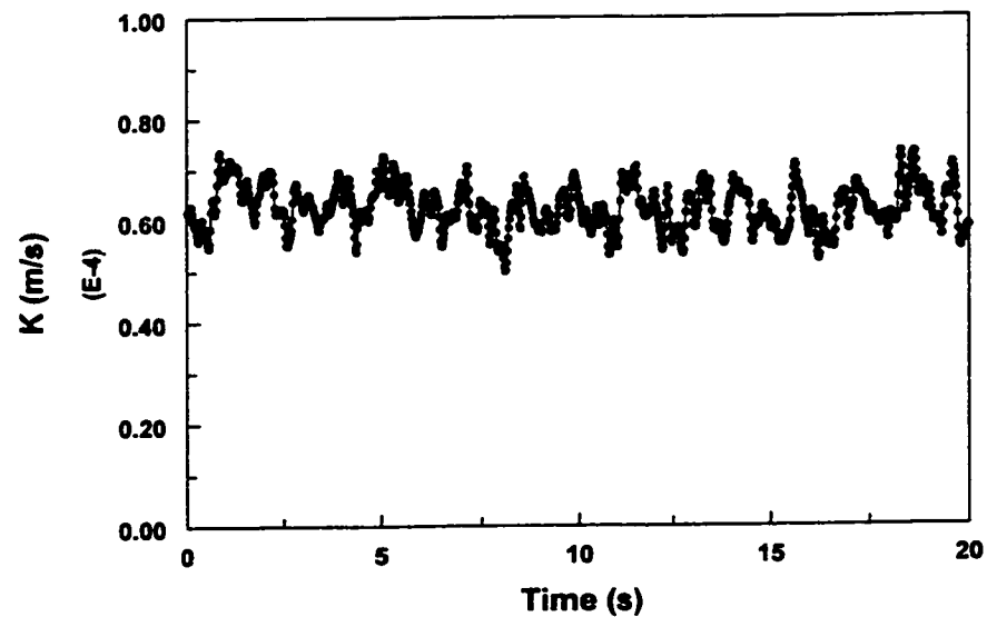
Figure 4.4.4 Instantaneous mass transfer coefficient in water/gas two-phase flow with V_{sl}=1.0 m/s and V_{sg}=0.6 m/s
