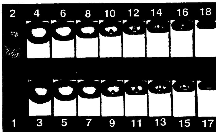
Figure 2.12 Series of photographs showing the development of the microjet in a bubble collapsing very close to a wall (Tomita and Shima, 1990)
